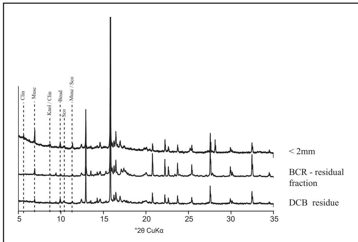
Figure III.6. Example of XRD patterns performed on residual fractions after BCR treatment or after DCB extraction (<2mm fractions from Z_{ic} horizon, profile 1); clin, musc, kaol, beud, sco, qtz refer respectively to clinocllore, muscovite, kaolinite, beudantite, scorodite, and quartz.
