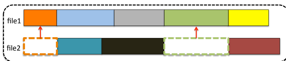
Figure 1.4: Deduplication Example
