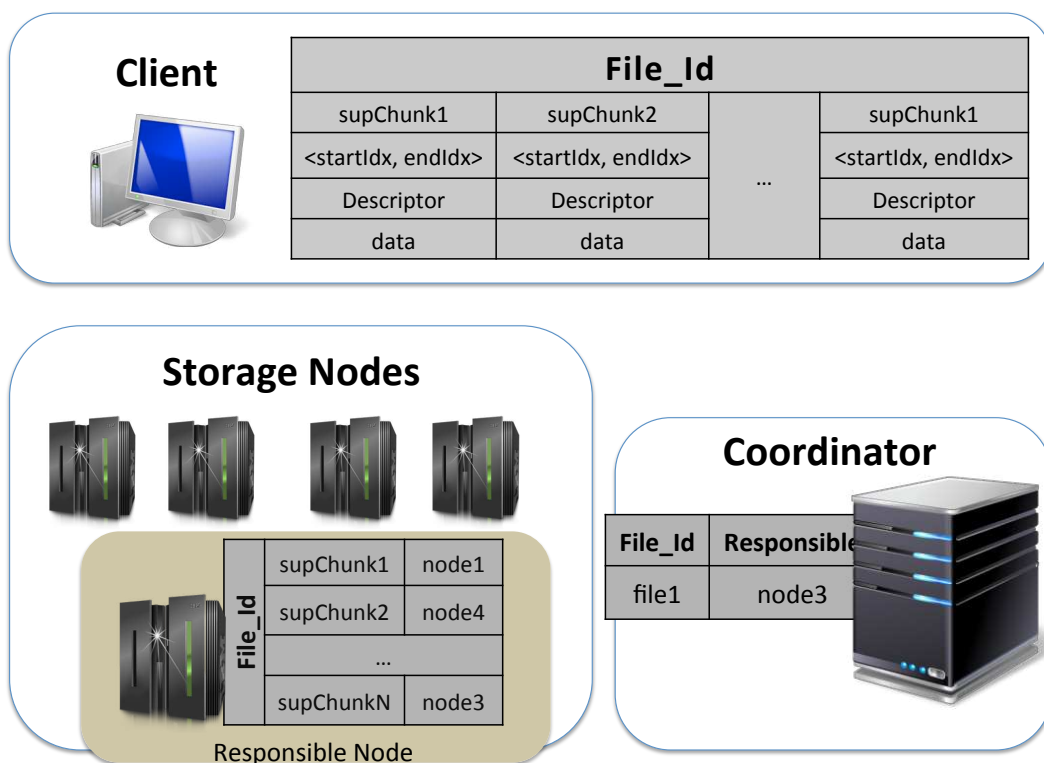
Figure 2.5: System Architecture
