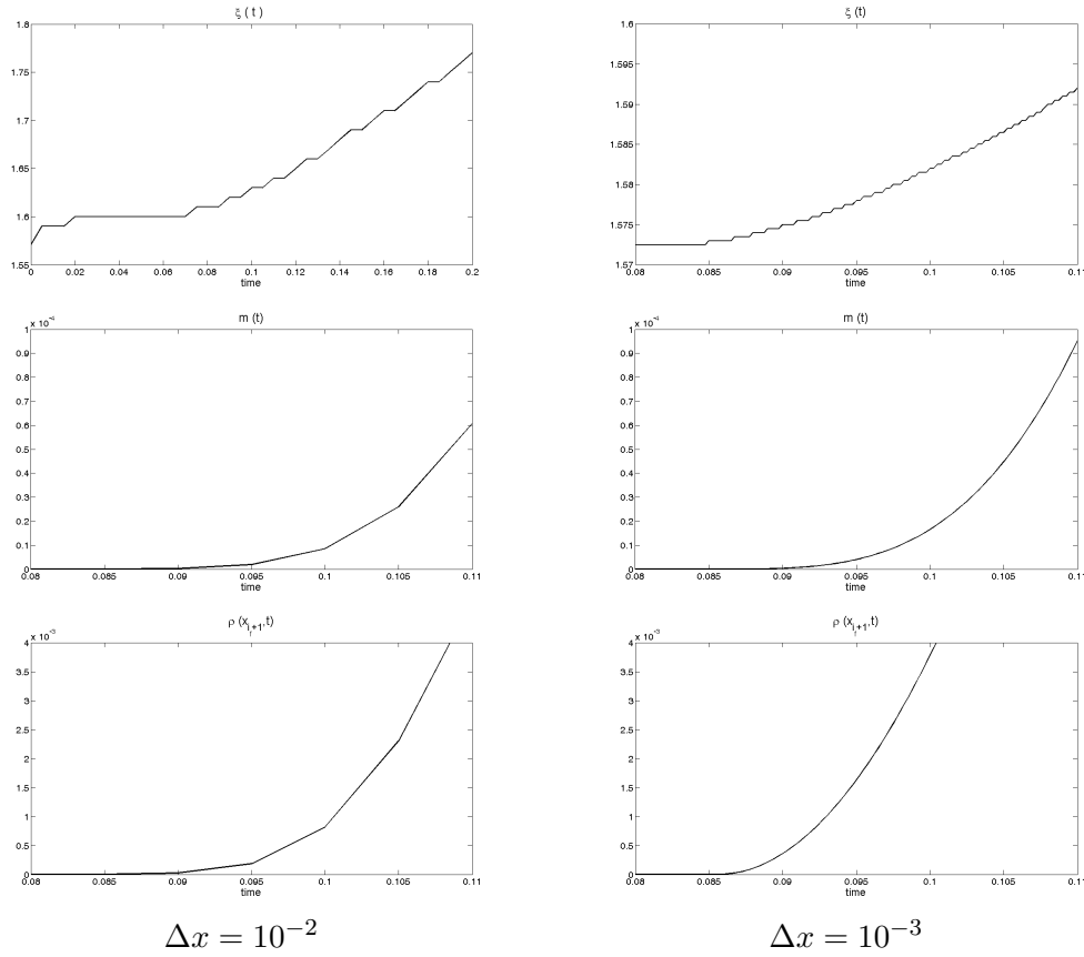
Figure 5.1: Porous medium equation: time evolution of the interface \xi(t) , the mass m(t) in (x_f, L] and the value of density \rho_{i_f+1}(t) for the space step \Delta x = 10^{-2}, 10^{-3} . Comparison of the criteria determining the waiting time t^* . The exact value is t^* = 0.083 .
