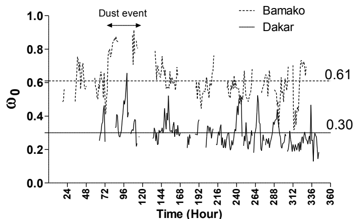
Figure S1: Temporal evolution of single scattering albedo ( \omega_0 = \sigma_{\text{scat}} / (\sigma_{\text{abs}} + \sigma_{\text{scat}}) ) in Bamako and Dakar.
