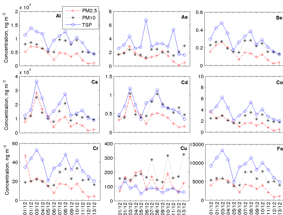
Figure 7: Time variations of components in PM_{2.5} , PM_{10} and TSP concentrations measured at Dakar between 01 and 13 December 2009.
