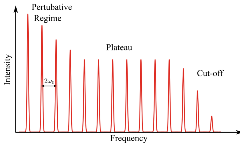
Figure 1.1.: Typical structure of a high order harmonic spectra generated in a gas (figure adopted from (Higuët, 2010)).
