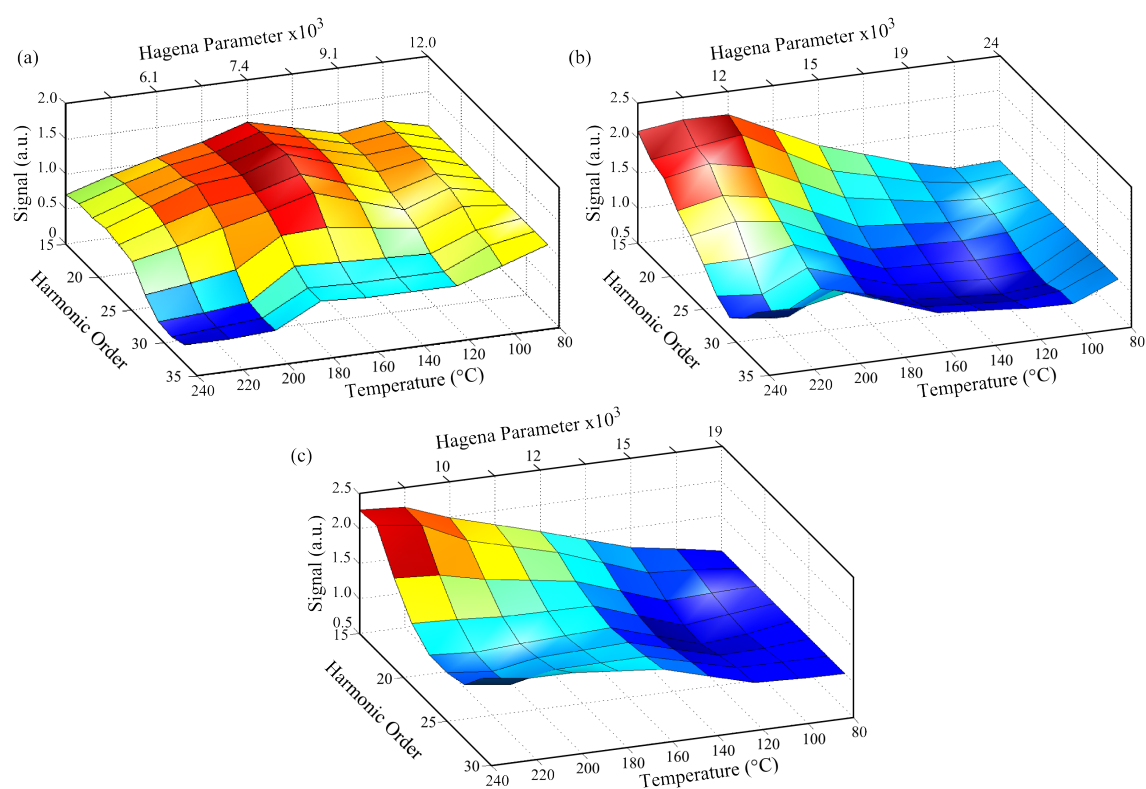
Figure 4.6.: Total signal of different harmonics as a function of temperature normalized to its value at 80 °C. HHG are generated in carbon dioxide at a backing pressure of (a) 10 bar, (b) 20 bar and (c) in krypton at a backing pressure of 20 bar.
