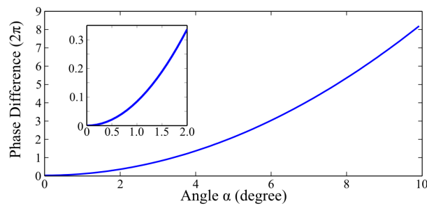
Figure 4.28.: Phase difference between the ordinary and extraordinary beam as a function of AOI on the \text{MgF}_2 plate.
