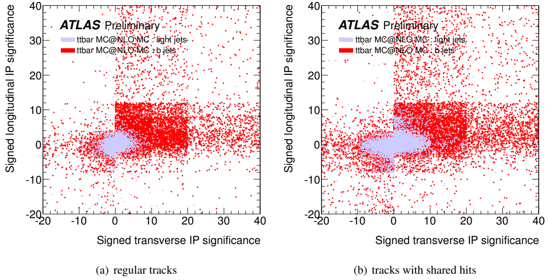
Figure 3.26: Signed track impact parameter significances z_0/\sigma_{z_0} versus d_0/\sigma_{d_0} reference distributions for the IP3D algorithm for regular tracks (left plot) and for tracks with shared hits (right plot), obtained from simulated t\bar{t} events.
