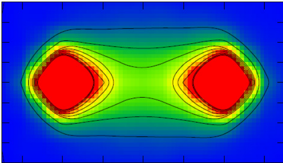
Figure 2.11: (top) Modelisation of the coupling between two quarks as a color flux tube. (bottom) Result from lattice QCD simulation of a quark and antiquark (red) 'glued' together (green) [87].
