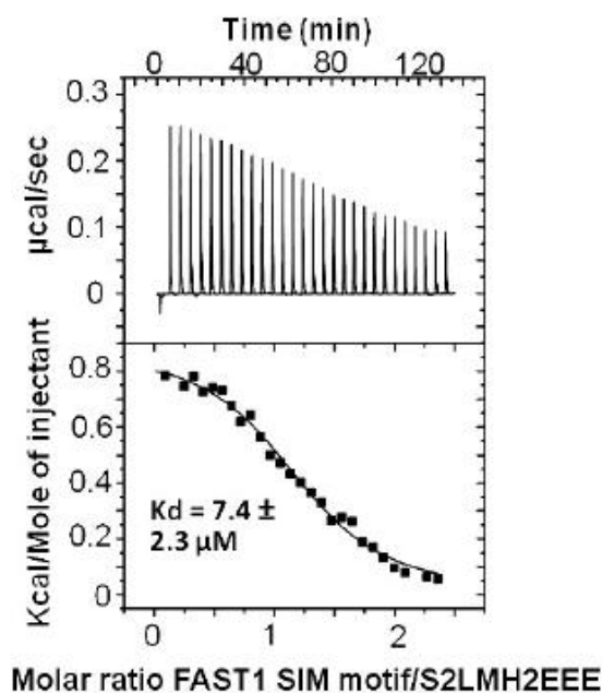
Figure 3S: Binding curve obtained by ITC for FAST1 peptide LDALFQGVPPNKSIYDVVWVSHPRDL added to a phosphomimetic mutant of the MH2 domain of Smad2 (S2LMH2EEE).
