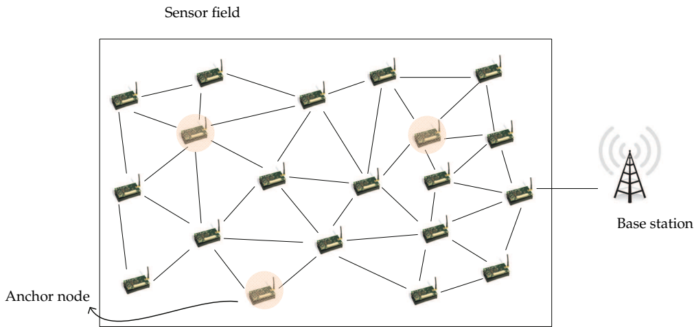
Figure 4.1: A wireless sensor network scenario
