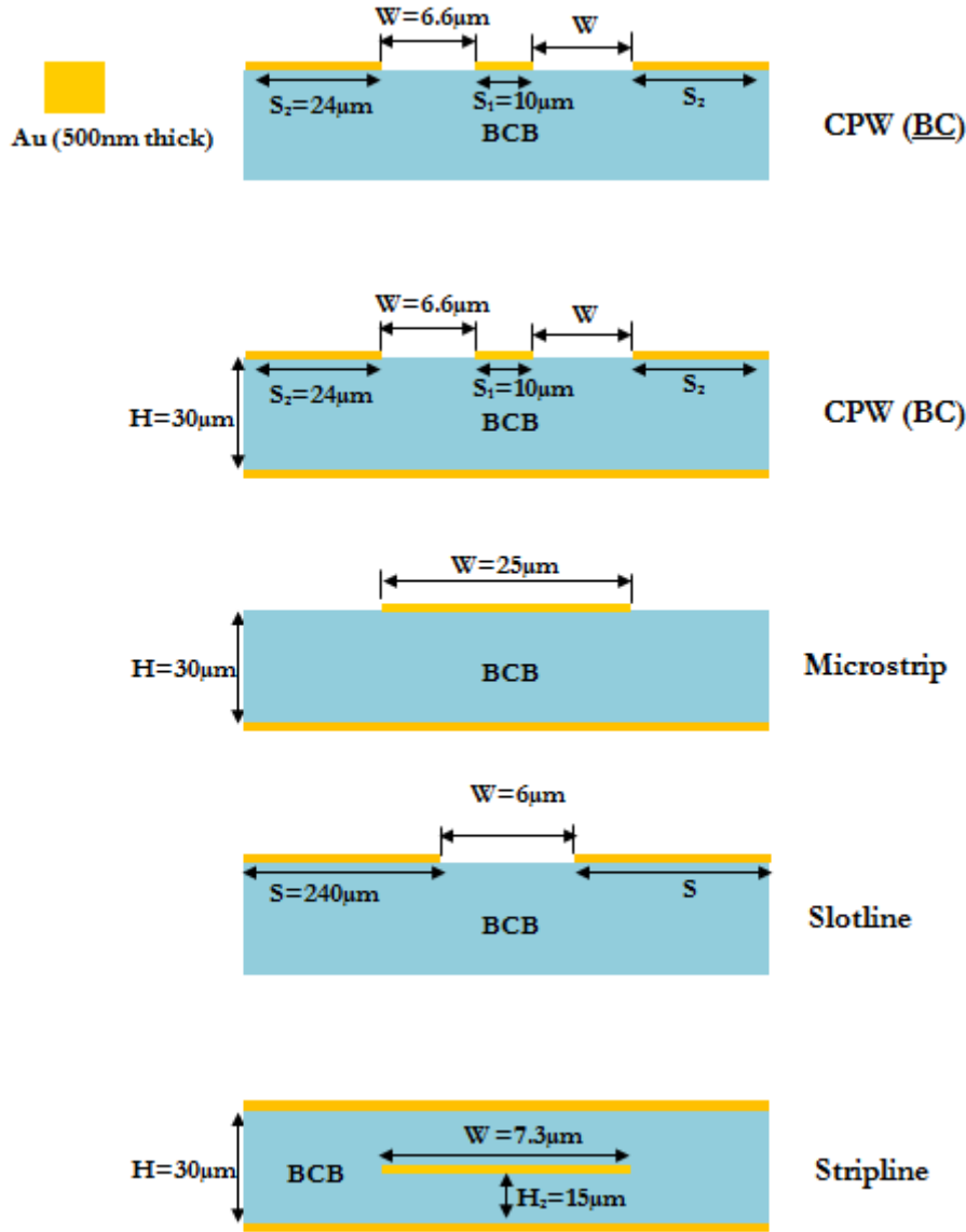
Figure 3-41: Dimensions of different 100 Ω waveguides for comparisons
