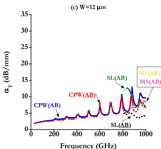
Figure 3-9: Influences of airbridges (AB) on the total attenuation of mode CPW, Slotline (SL) and Microstrip (MS) for CPW on 30 \mu m BCB with backed conductor: (a) W = 1.6 \mu\text{m} , (b) W = 6.6 \mu\text{m} and (c) W = 12 \mu\text{m}
