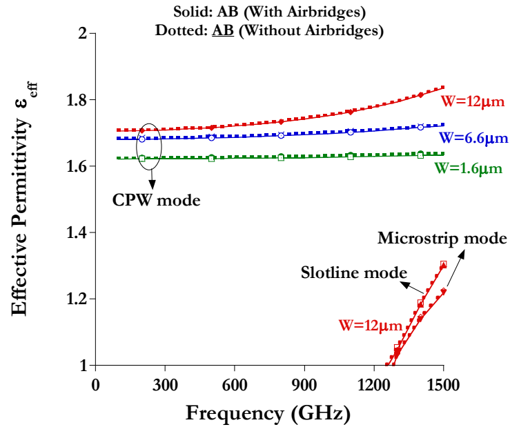
Figure 3-8: Influences of airbridges (AB) on the effective permittivity of the mode CPW, slotline and microstrip for CPW on 30\mu\text{m} BCB with backed conductor at different W
