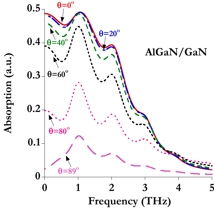
Figure 2-19: Original absorption of the heterostructure AlGaIn/GaN (3 \mu m) at room temperature with different incident wave angles by HFSS
