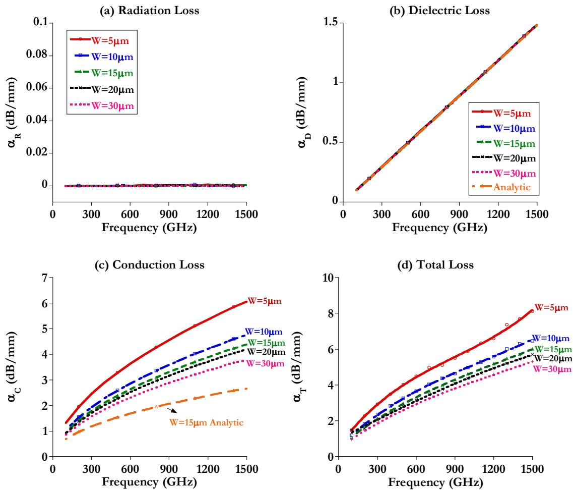
Figure 3-31: CST calculated losses of stripline in homogeneous 30 \mu\text{m} BCB, (a) Radiation loss, (b) Dielectric loss, (c) Conduction loss ( \sigma_{\text{Au}} = 5.10^6 \text{ S/m} ) and (d) Total losses ( \sigma_{\text{Au}} = 5.10^6 \text{ S/m} )
