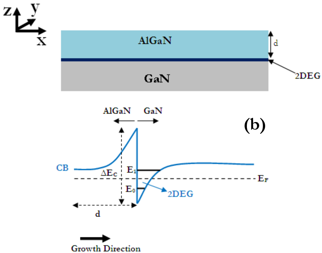
Figure 2-2: AlGaN/GaN heterojunctions (a) and the conduction band diagram (b)
