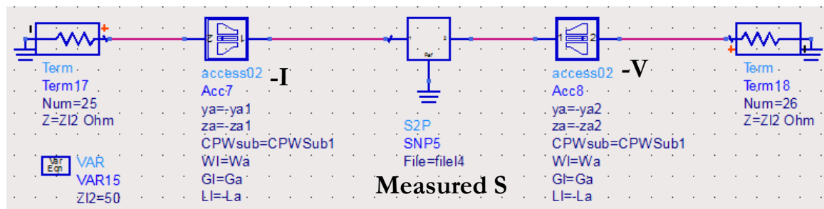
Figure 3-60: Circuit model for extracting the S parameters of CPW line ( S_1 = 36 \mu\text{m} , W = 3 \mu\text{m} ) based on measurement results and fitted transition models
