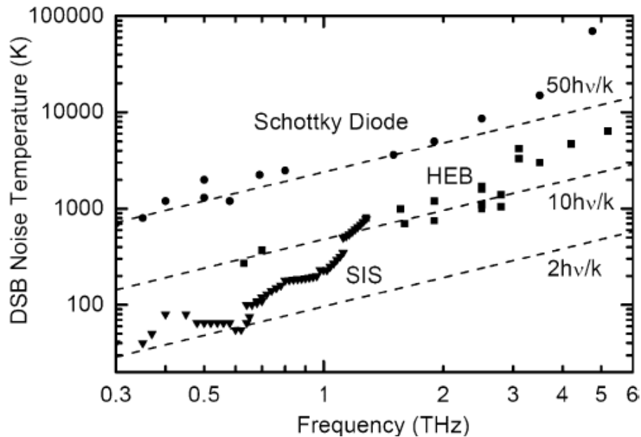
Figure 1-5: Noise temperature of heterodyne THz detectors [Hübers2008]
