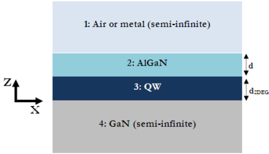
Figure 2-13: Screened and unscreened multi-layers structure with finite thickness 2DEG
