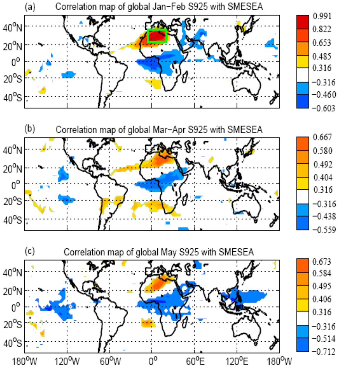
Figure 4.61: Map of significant correlation between south of the Mediterranean Sea (SMEESEA) specific humidity index and global S925 for (a) January–February, (b) March–April and (c) May. The green rectangle in (a) shows the approximate location of SMEESEA specific humidity index computed for January–February period from 1962 to 2000
