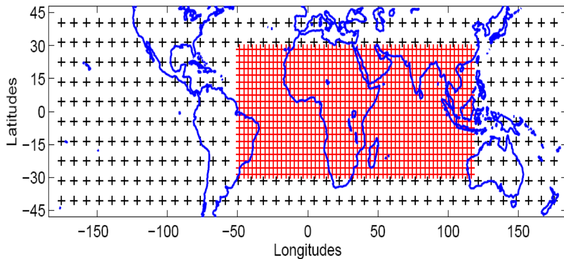
Figure 3.6: Map showing the nesting of the SST grid points. Red plus (+) are the fine grid resolution while the black plus (+) are for the coarse grid resolution.
