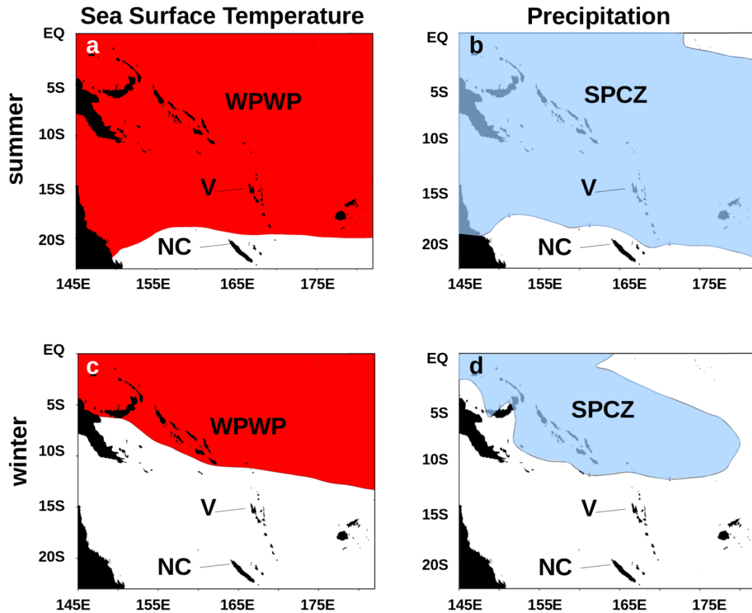
Figure IV-2. Seasonal location of the main climatic features of the Southwest Pacific. The Western Pacific Warm Pool (WPWP) is delimited by the 28^{\circ}\text{C} isotherm (red area - HadISST1 mean 1980-2011 period, (Raymer et al. 2006)). The South Pacific Convergence Zone (SPCZ) is delimited by the 6\text{ mm}\cdot\text{d}^{-1} isohyet (blue area - CMAP 1980-2010 (Xie and Arkins, 1997)). a and b - Austral summer settings (January, February, March) c and d - Austral winter settings (July, August, September). Vanuatu archipelago (V) and New Caledonia (NC) location are shown on each map. Modified from Climate Explorer ( http://climexp.knmi.nl ).
