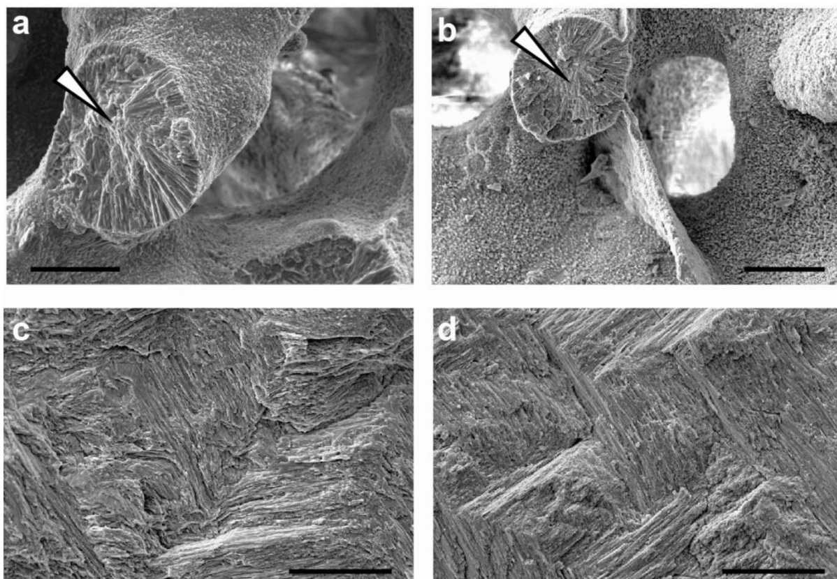
Figure III-4. Microstructural comparison between modern and fossil (this study) corals and giant clam (SEM images, scale: 50 \mu m). Massive coral Porites sp. specimens: (a) modern coral VA EPI; (b) early mid-Holocene coral Psp-07-09, with arrow indicating center of calcification. Giant clam Tridacna maxima specimens: (c) modern giant clam T-02-09; (d) early mid-Holocene giant clam T-10-09 (scale 50 \mu m).
