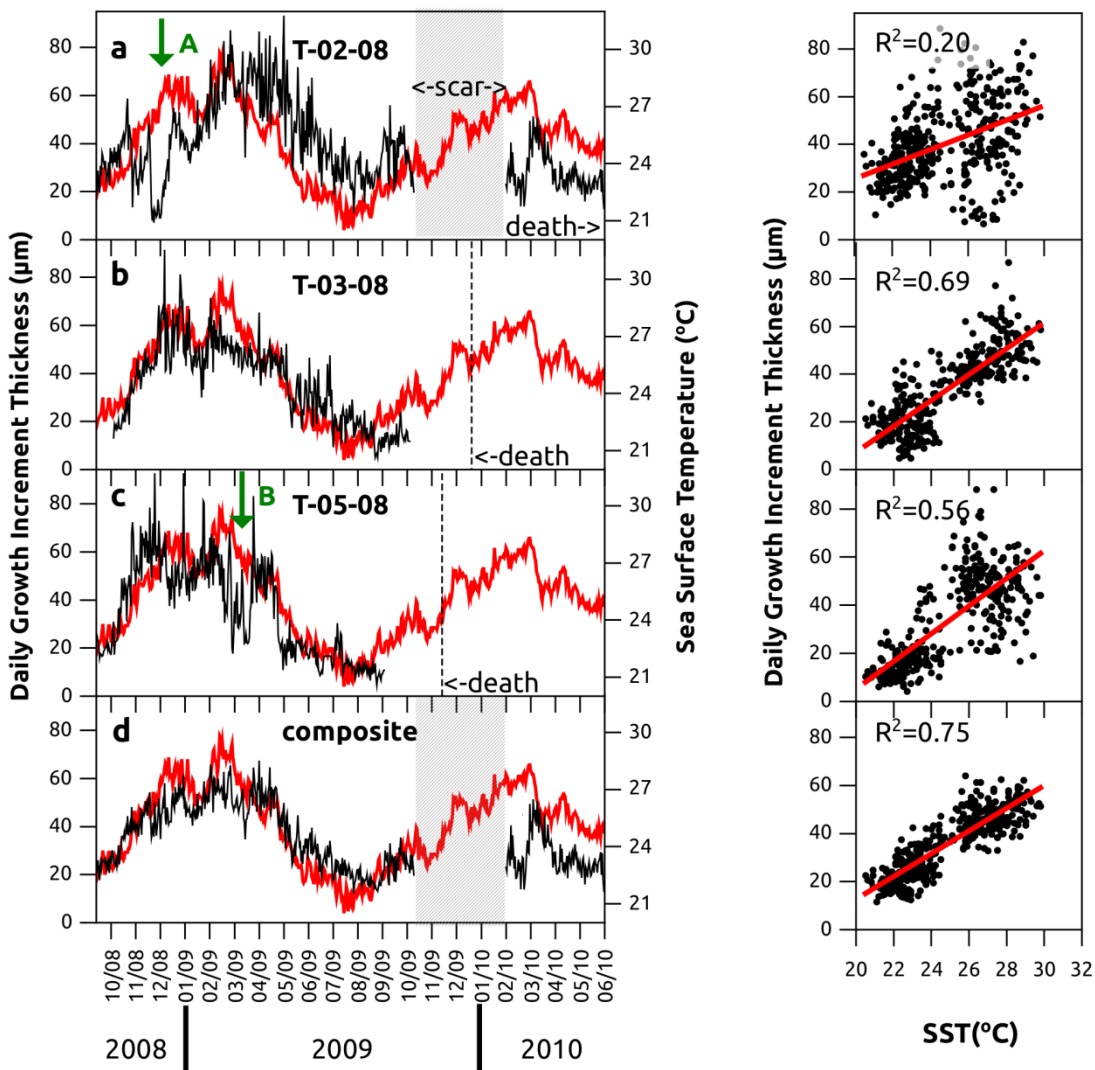
Figure II-6. Sclerochronological profiles of the three modern Tridacna maxima shells (black) together with the SST variations (red). Regressions between daily increment thickness and SST are shown on the right of each profile. The R^2 values are significant at a 95% threshold. a to c - T-02-08, T-03-08, and T-05-08. d - Composite profile. For T-02-08 and the composite profile, regressions did not include the data after the scar. Dotted lines indicate the date of death of the specimens. Anomalous growth events A and B are shown by green arrows (see text for details).
