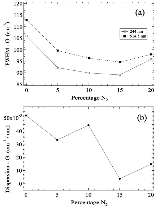
FIG. 4. (a) FWHM of the G peak for UNCD films as a function of nitrogen addition in the synthesis gas. (b) Dispersion of the G peak for these UNCD films.
