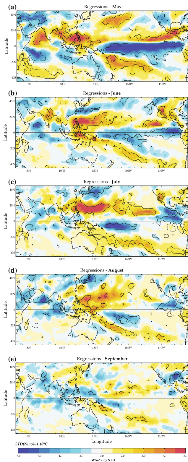
Fig. 4 Regression of Nino(−1) index onto monthly OLR anomalies from May to September. Regressions that are above the 90% confidence level estimated with a phase-scrambling bootstrap test with 999 sampled are encircled . The standard deviation of the Niño3.4 index is given at the bottom of the panels
