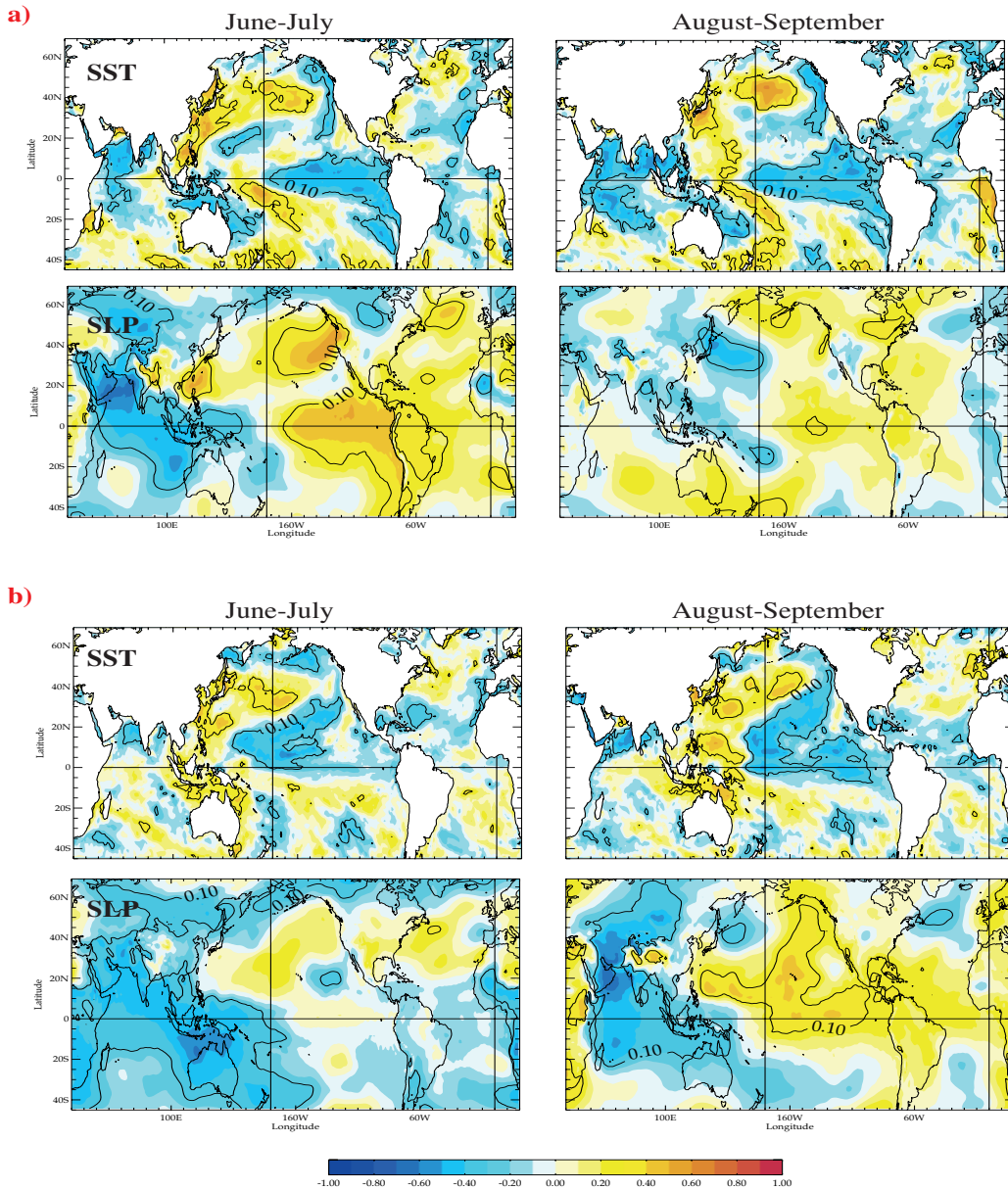
Figure A.4: Correlation of summer SST ( top panels ) and SLP anomalies ( bottom panels ) with a) ISM rainfall in JJ and b) ISMR rainfall in AS, during El Niño years selected in the SINTEX-F control simulation (upon a 0.5 standard deviation of the Niño3.4 SST index in December-January). Correlations significant at the 90% confidence level according to a two-tailed student-t test are encircled.
