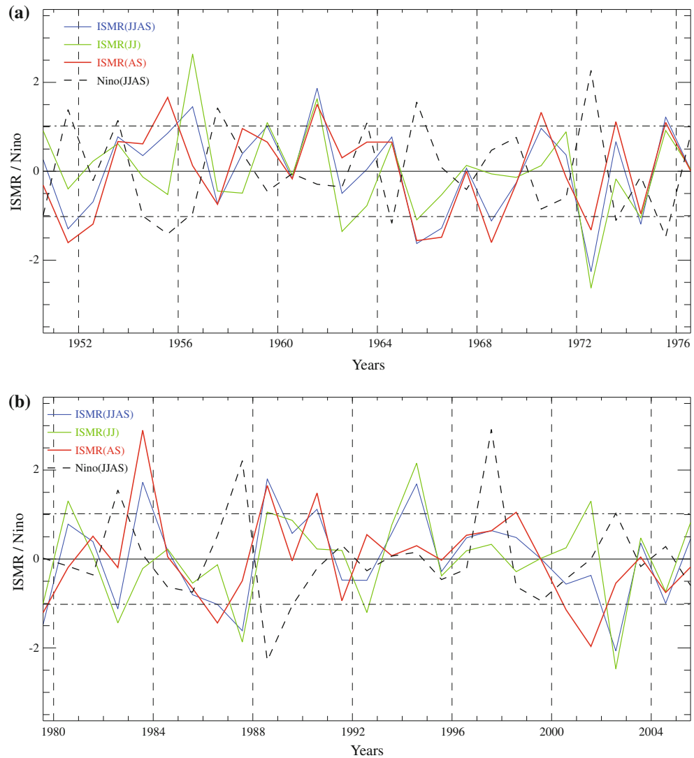
Fig. 2 Standardized time series of ISM rainfall in JJAS ( blue curve ), JJ ( green curve ) and AS ( red curve ) superimposed with the standardized Niño3.4 time series in JJAS ( black dotted curve ) during a 1950–1976 and b 1979–2006. The one standard deviation line (in black ) is also added to this figure as it helps identify the extreme years
