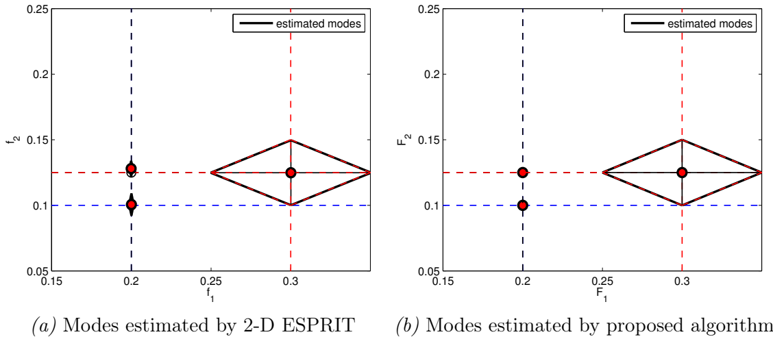
FIGURE 4.5 – Comparison between 2D-ESPRIT and the proposed method with \text{SNR}_1 = 20 dB. ( \circ ) Frequencies of simulated 2-D modes; ( \bullet ) Frequencies of estimated 2-D modes; ( \diamond ) The diagonals of the diamonds represent the 2-D damping factors.
