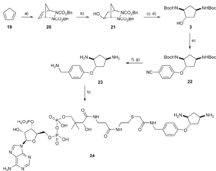
Scheme 3. a) DBAD, \text{CH}_2\text{Cl}_2 , quantitative; b) CatBH, 1% [\text{Rh}(\text{COD})\text{Cl}]_2 , 2% ( R,R )-BDPP, DME, -50^\circ\text{C} then \text{H}_2\text{O}_2 , 77%, ee = 83%; c) \text{H}_2 , \text{PtO}_2 , AcOH, quantitative; d) \text{Boc}_2\text{O} , NaOH 88% from 21; e) p -fluorocyanobenzene, KHMDS, 4^\circ\text{C} to RT, 68%. f) \text{H}_2 , 10% Pd/C, MeOH, 18 h; g) HCl, AcOEt, 10 min., 73% from 22; h) Auclair's procedure (ref. [4]), preparative HPLC purification, 40%.
