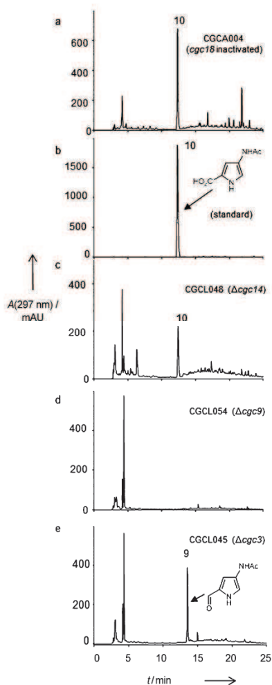
Figure 2. LC analysis of culture supernatants of mutants with deletions in congenicidin biosynthetic genes. Chromatograms from a) CGCA004 (disruption of cgc18 ); b) synthetic 10 ; c) CGCL048 ( \Delta cgc14 ); d) CGCL054 ( \Delta cgc9 ), and e) CGCL045 ( \Delta cgc3 ).
