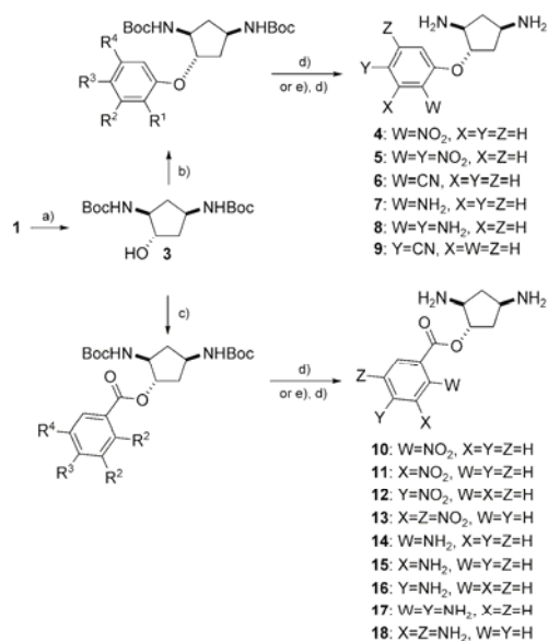
Scheme 2. a) \text{Boc}_2\text{O} , NaOH, dioxane/ \text{H}_2\text{O} , 84%; b) KHMDS, THF, ArF, 66–88%; c) DCC, cat. DMAP, \text{CH}_2\text{Cl}_2 , ArCOOH, 47–66%; d) HCl (gas), AcOEt, quantitative; e) \text{H}_2 , 10% Pd/C, AcOEt or THF, 43–93%.
