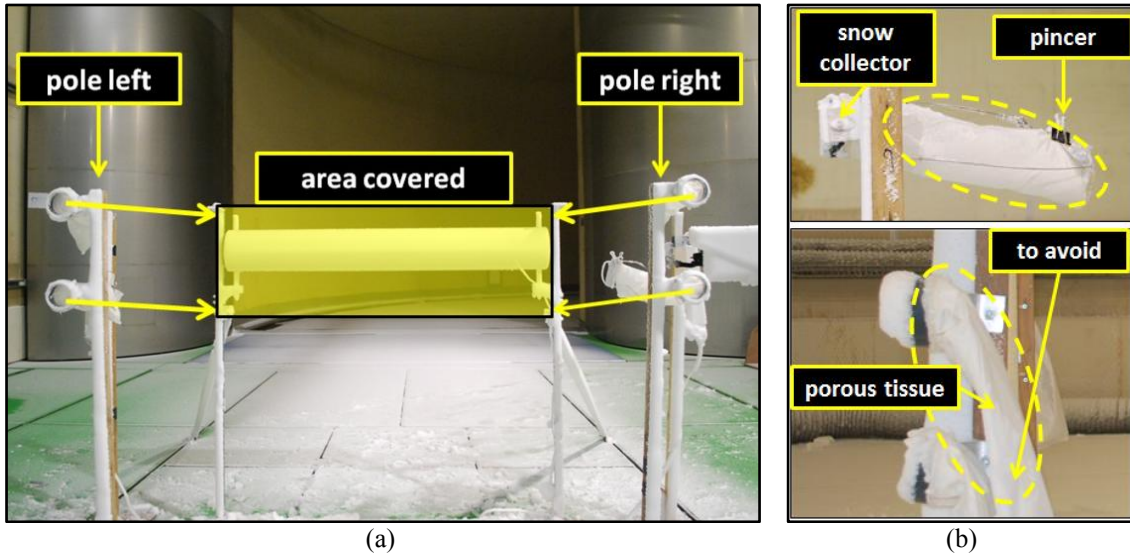
Figure 41. (a) Front view of the test structure with the four snow collectors. (b) Fide view of the snow collectors.
