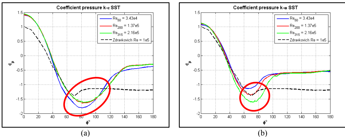
Figure 119. Pressure coefficient (a) k - \varepsilon model. (b) k - \omega SST model.
