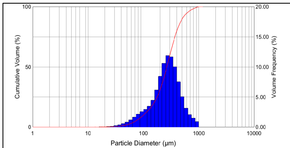
Figure 88. The PSD supposed at the exit of the snow gun [9]
