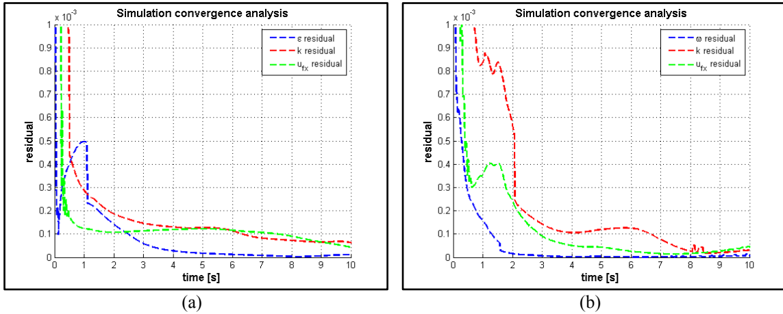
Figure 118. Convergence analysis (a) k - \varepsilon model. (b) k - \omega SST model.
