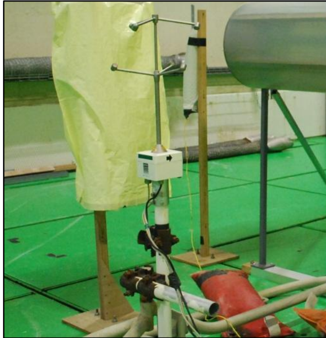
Figure 49. The ultrasonic anemometer on its support.
