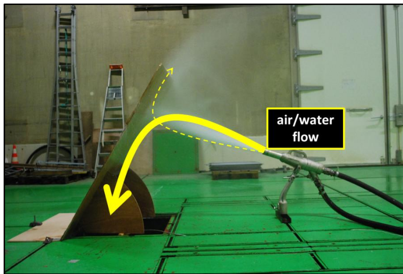
Figure 38. Function principle of the trapdoor.
