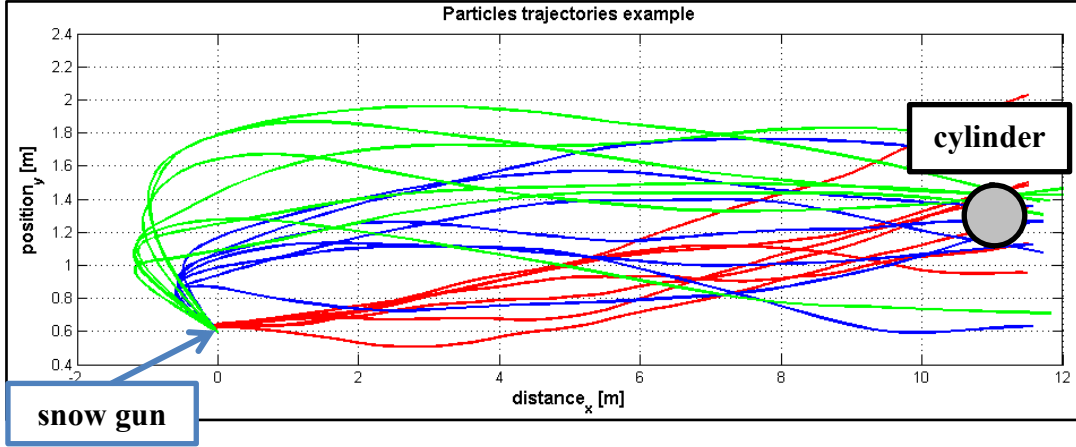
Figure 86. Particle trajectories example: red d_p = 40\mu\text{m} , blue d_p = 260\mu\text{m} , green d_p = 520\mu\text{m} .
