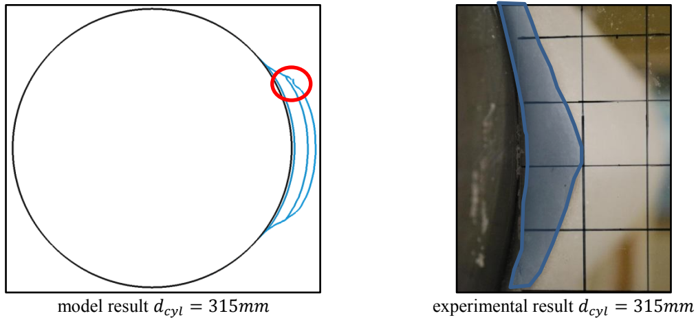
Figure 142. Accretion shapes obtained.
