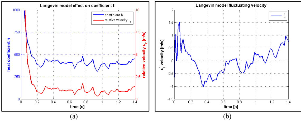
Figure 100. (a) Effects of Langevin model on u_r and h , (b) u_f' example.
