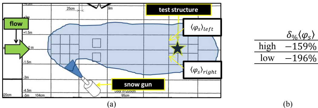
Figure 58. (a) Configuration with one side snow gun. (b) \delta_{0\%} \langle \varphi_s \rangle differences.
