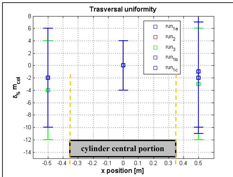
Figure 70. Impacting flow uniformity on the cylinder central portion.
