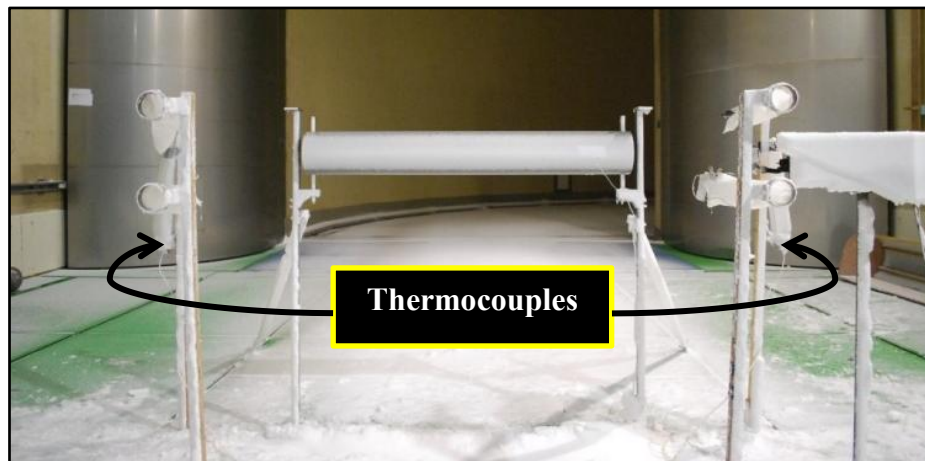
Figure 45. Thermocouples position.
