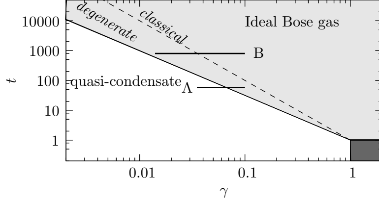
Figure 58: Phase diagram of the one dimensional Bose gas, in (\gamma, t) coordinates. The two segments [\gamma_m, \gamma_M] show the positions of the two sets of data analyzed in this chapter. \gamma_m corresponds to the peak density of the in situ profile, the segment is such that 80 % of the atoms lie in a region of density larger than that associated to \gamma_M .
