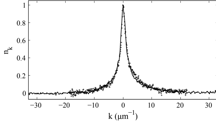
Figure 62: Momentum distribution of a gas of 7000, atoms at thermal equilibrium in a 7.5 Hz longitudinal trap and 4.6 kHz transverse trap. The solid line is the momentum distribution obtained without the levitation step, with a free fall time of 24.7 ms. The dots are the momentum distribution of the same sample, obtained with a levitation time of 20.6 ms followed by a free fall time of 22.7 ms.
