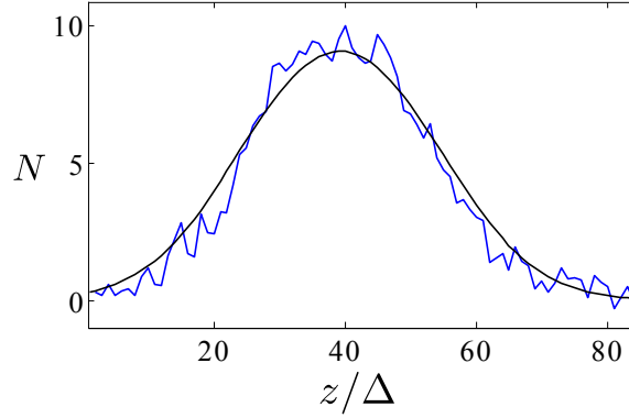
Figure 43: Longitudinal density profile of 300 atoms in a ( f_{//} = 5.6 Hz, f_{\perp} = 56 kHz) trap. A fit of the Yang-Yang theory (solid line) to the data gives t = 0.4 . At the center of the trap, we find \gamma = 2.6 .
