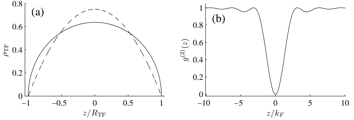
Figure 11: (a) Zero temperature density profile of a 1D Bose gas in a harmonic trap : in the 1D mean field regime (dashed line), and in Tonks regime (solid line). The profiles are normalized to the same integral, and the horizontal axis is rescaled for each profile with the corresponding Thomas-Fermi radius. (b) Two body correlation function of a Tonks gas at zero temperature.
