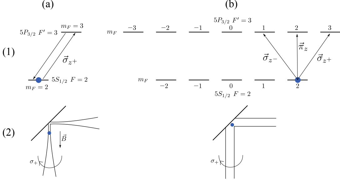
Figure 33: (a) (1) Closed imaging transition obtained in the case where a purely \sigma_+ polarized light is sent on the cloud. In the experiment, if the cloud is far enough for the chip surface, it can be obtained by focusing the beam on the cloud (2, a). (b) (1) In the case of a non purely polarized light all the transitions have to be considered, together with the Zeeman shifts which are different for upper and lower levels. This happens if the cloud is too close to the chip, so that it is reached by both incident and reflected light (2).
