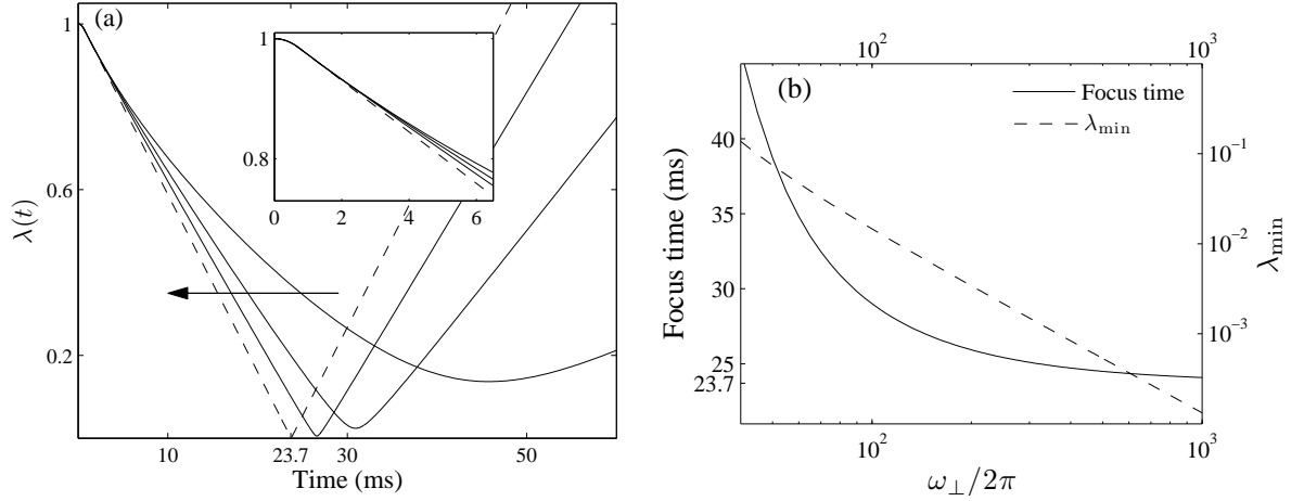
Figure 60: (a) Evolution of the scaling parameter \lambda(t) for the sequence of Fig. 45, for \omega_{//} = 8 Hz, \tau_1 = 30\mu\text{s} , \tau = 690\mu\text{s} , \omega_f = 40 Hz, and for the following values of \omega_{\perp} : 40 Hz, 80 Hz, 160 Hz (solid lines). The arrow points in the direction of increasing \omega_{\perp} . The dashed line is the limit of Eq. 302 where interactions are switched off instantaneously. For very large \omega_{\perp} , the curves converge towards this limit which gives a focusing time of 22.1 ms. The inset is a zoom around t = 0 . (b) Focus time (solid line) and value of \lambda at the focus time versus \omega_{\perp}/2\pi .
