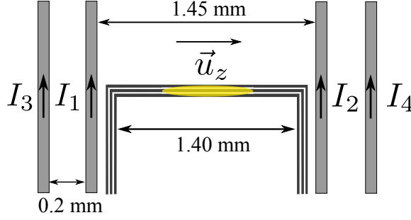
Figure 50: Wire configuration. The cloud is represented in yellow, and its longitudinal axis is \vec{u}_z . The modulated guide has a length of 1.4 mm, and there are four wires perpendicular to it, for longitudinal confinement. Those wires are running the DC currents I_1 , I_2 , I_3 and I_4 .
