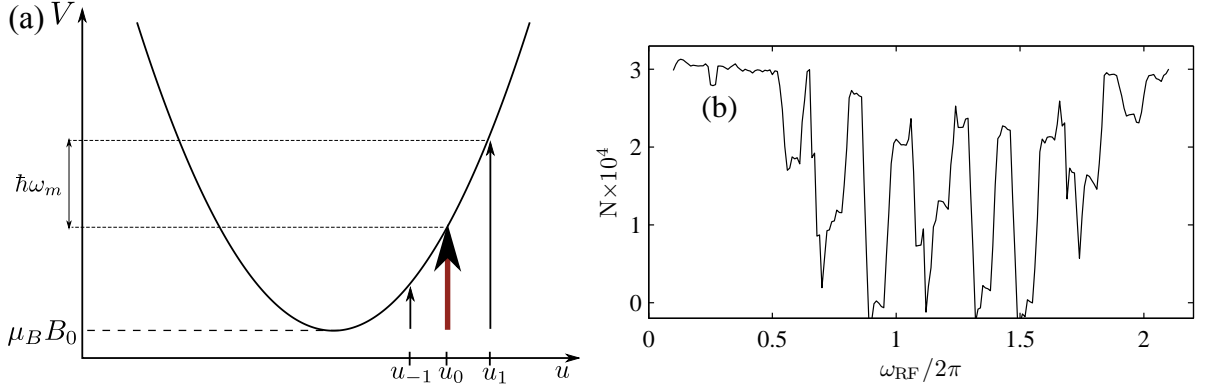
Figure 22: (a) Transverse potential. The carrier and two sidebands are represented. Each sideband is an additional knife. (b) Atom number in the modulated guide monitored after a hold time in the presence of a radio-frequency field.
