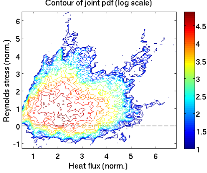
Figure 4.7: Logarithmic contour of the joint statistical distribution of turbulent heat flux and Reynolds stress. Both fluxes are normalized to their respective standard deviations.
