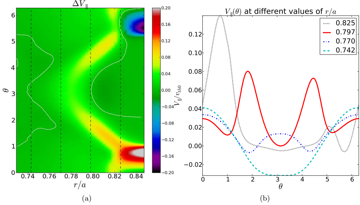
Figure 5.9: Effect of a boundary condition with V_{||}/v_{th0} = 0.25 at \theta = +\pi/4 . (a) Modification of the poloidal structure of parallel velocity near the edge, and (b) poloidal profiles at several radii, indicated with dashed black lines in (a).
