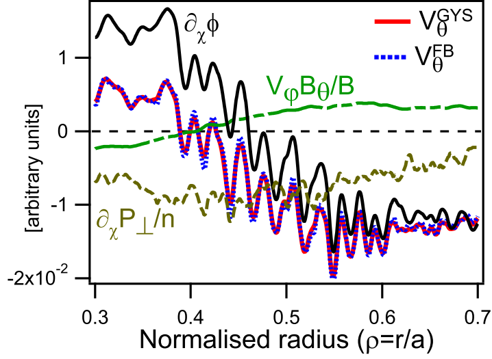
Figure 3.1: Numerical test of the radial force balance, comparing the poloidal velocity as computed directly in the code ( v_\theta^{GYS} ) and as a sum of the other terms in the radial force balance equation ( v_\theta^{FB} ).
