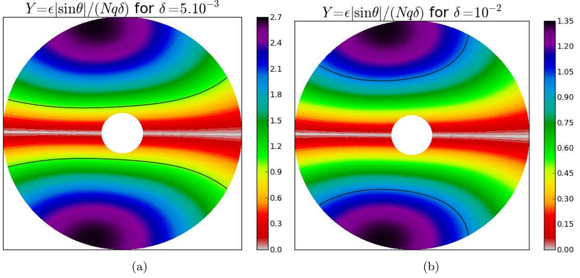
Figure 6.2: Poloidal cross-sections of the condition for local trapping in the ripple perturbation with the parameters: R_0/a = 3.2 , N = 8 and (a) \delta = 5.10^{-3} or \delta = 10^{-2} . Local trapping occurs when Y < 1 , corresponding to the domain between the two black lines.
