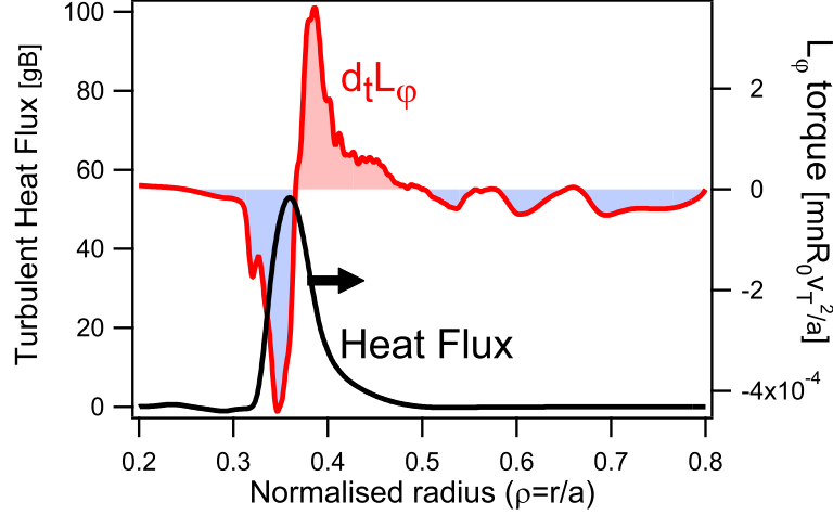
Figure 4.1: Propagation of a front of turbulent heat flux and generation of toroidal rotation. The turbulent heat flux is in gyro-Bohm units (see section 5.2).
