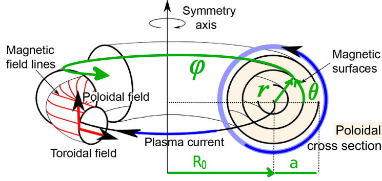
Figure 2.1: The tokamak magnetic configuration and the toroidal coordinate system (r, \theta, \phi) . The geometry of the torus can be described by its minor radius a and major radius R_0 (at the magnetic axis)
