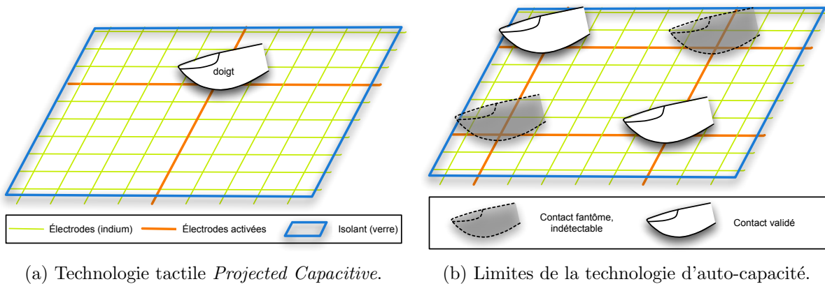
FIGURE 1.11 – Illustrations de la technologie tactile capacitive.
