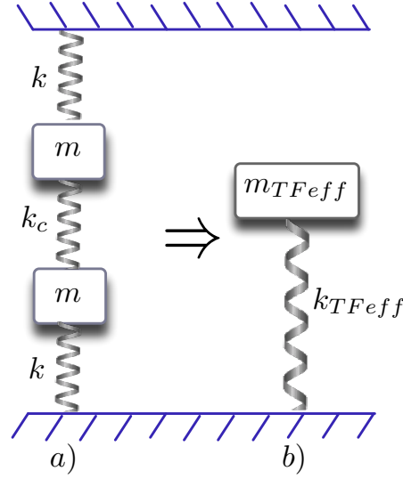
Figure 1.15 - Schematic diagram of tuning fork coupled oscillators model with noncontact
