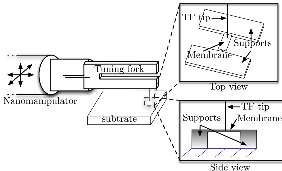
Figure 3.15 - System configuration for membrane stiffness characterization
