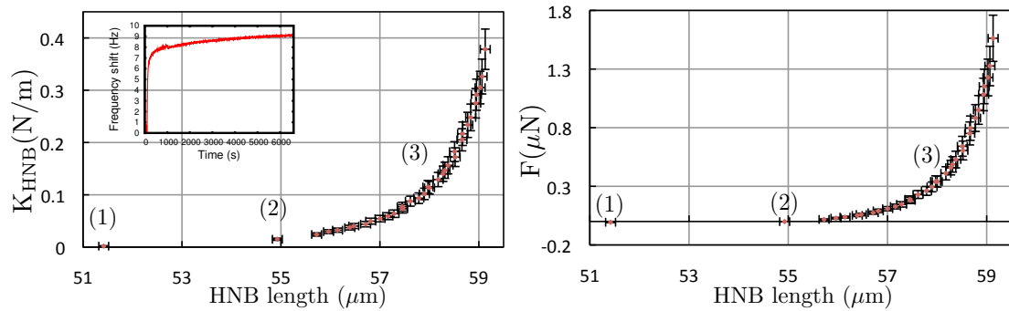
(a) HNB longitudinal stiffness. Inset: Frequency shift recorded during pumping of the SEM chamber
