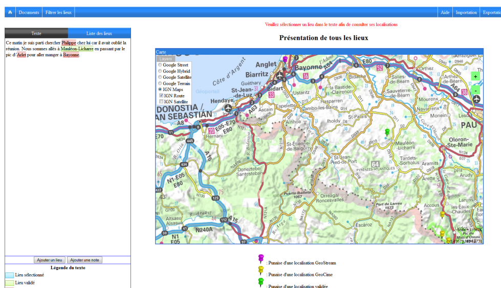
FIGURE 5.35 – Projet GeoText2Map
