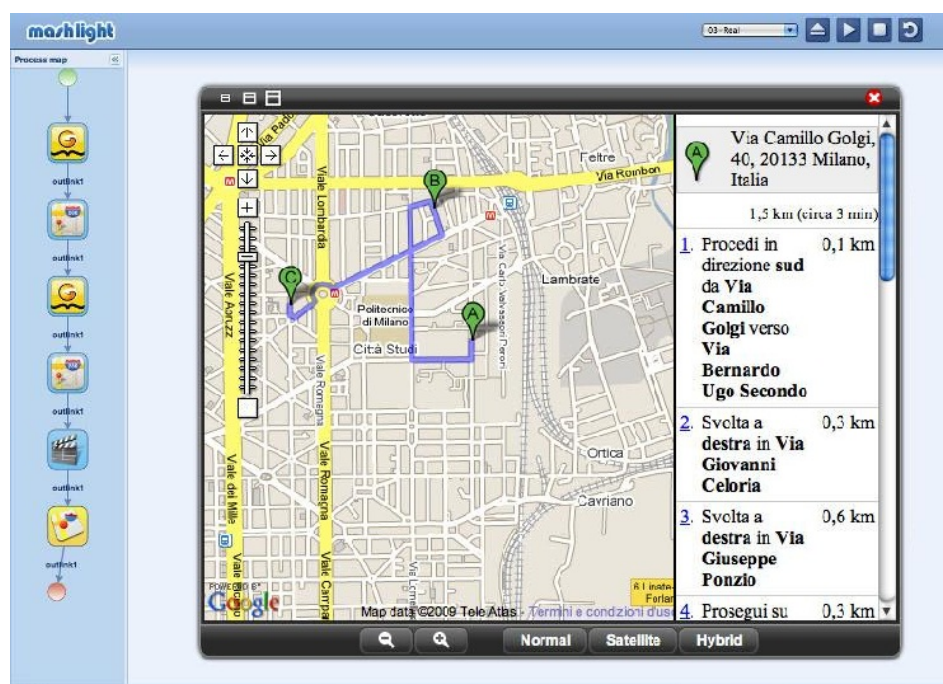
FIGURE 3.18 – Interface de Mashlight
