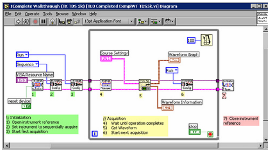
FIGURE C.6 – Langage de programmation LabVIEW
