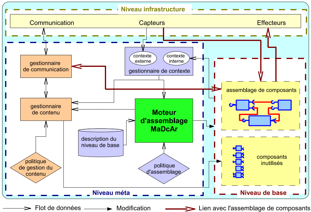
FIGURE 5.1 – Architecture générale de MADCAR-AGENT.
