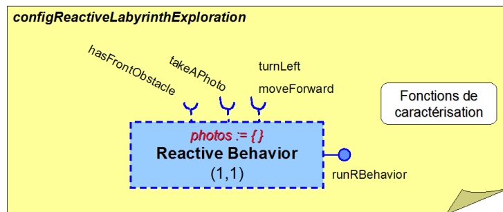
FIGURE 5.11 – Configuration configReactiveLabyrinthExploration.
