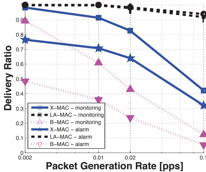
FIGURE 3.7 – Scenario 1, grid network with heterogeneous traffic. Delivery ratio of alarm and monitoring frames vs. packet generation rate. 100 nodes are deployed in a 10x10 grid ; alarm source has rank 10.
