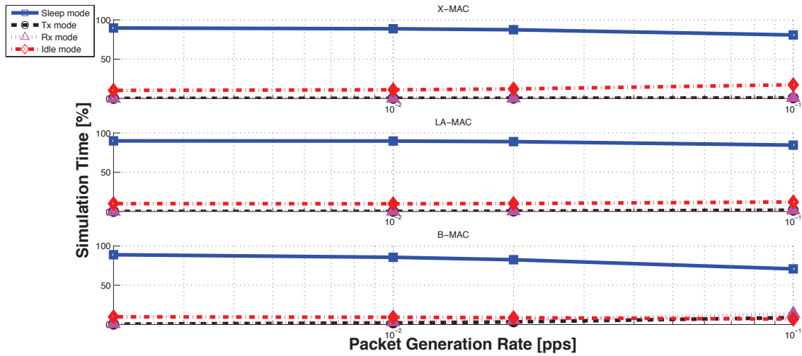
FIGURE 3.10 – Scenario 1, grid network with heterogeneous traffic. Percent ime spent in each radio mode versus the traffic load.
