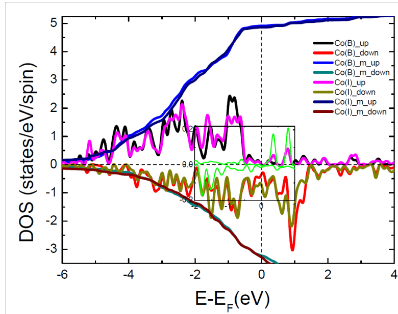
Fig. 4.4 : Spin-resolved density of states for bulk cobalt, Co(B), and interfacial cobalt, Co(I), are shown in graphene|Co systems. Their integral curves are also shown correspondingly. Inset is the density of states for the carbon atom on top of Co.
