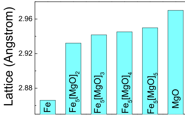
Fig. 2.2 : In plane lattice constant of [\text{Fe}_5(\text{MgO})_x]_2 as a function of MgO thickness.
