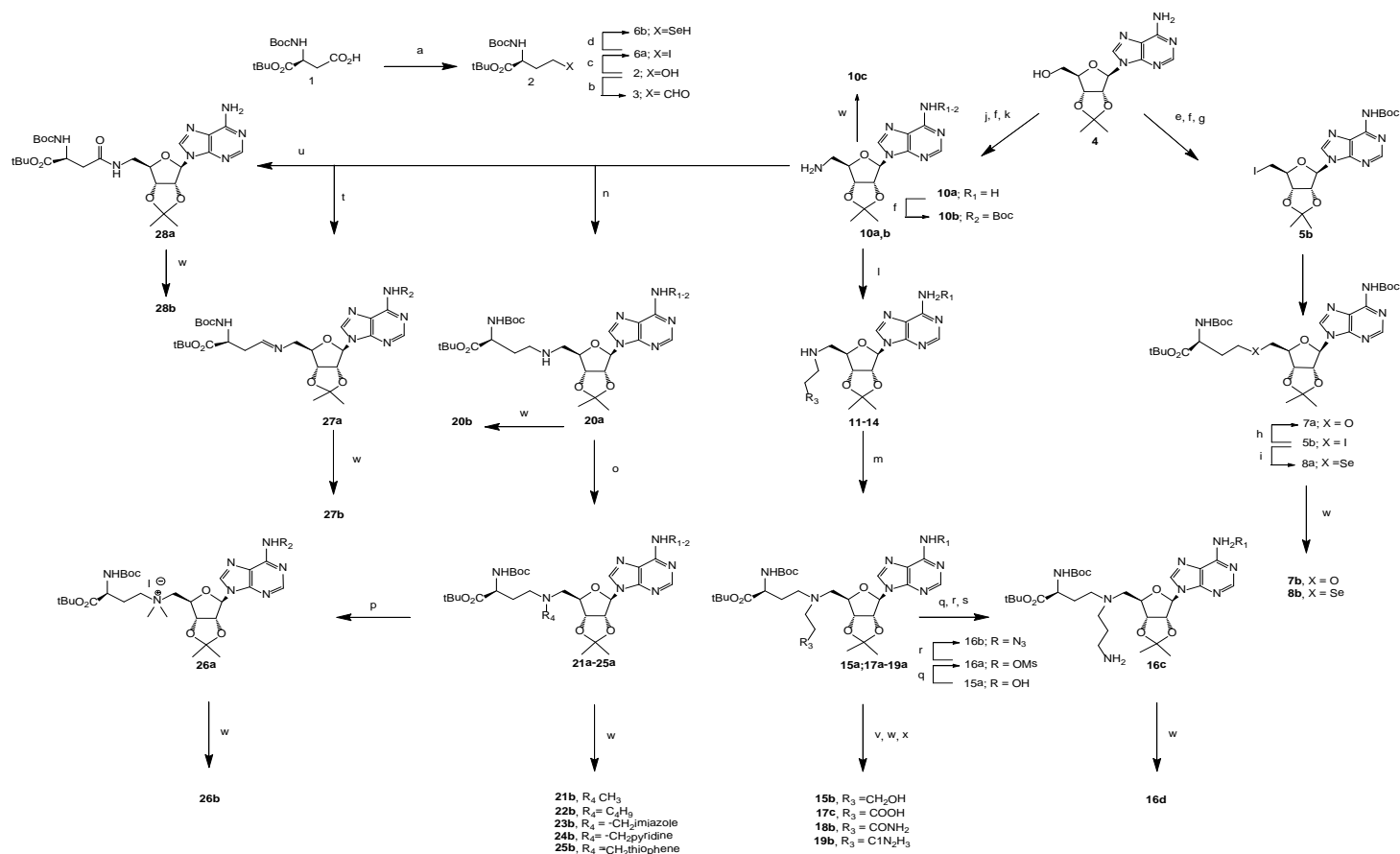
Scheme 1: Reagents and conditions: a) 1 , EtOCOCl, DIEA, THF, 45 minutes at -5°C, NaBH 4 , H 2 O, 12h at room temperature; b) 2 , Dess-Martin reagent, DCM, 6h at room temperature; c) 2 , I 2 , PPH 3 , imidazole, DCM, 3h at room temperature; d) Se (s), DMF, NaOH, N 2 H 4 , 3h at 60°C, then 6a , DMF, 18h at 60°C, NaBH 4 , EtOH, 2h at 0°C then 12h at room temperature; e) 4 , TsCl, pyridine, 6h at 0°C; f) Boc 2 O, NaH, THF/DMF, 12h at 60°C; g) NaI, acetone, 12h at 60°C; h) 2 , NaH, THF, K 2 CO 3 , 24h at 70°C; i) 6b , DMF, 12h at 80°C; j) 4 , DPPA, DBU, dioxane, 3h at room temperature, TBAI, NaN 3 , 12h at 110°C; k) H 2 /Pd/C, MeOH, 12h at room temperature; l) 10 a-b , R 3 X, DIEA, THF, 12h at 60°C; m) 3 , 11-14 , HOAc, NaBH 3 CN, MeOH, 12h at room temperature; o) 20a , R 4 CHO, HOAc, NaBH 3 CN, MeOH, 12h at room temperature; p) 21a , MeI, EtOH anhydrous, 6 days at room temperature; q) 15a , MsCl, DIEA, THF, 12h at room temperature; r) 16a , NaN 3 , CH 3 CN, 48h at 80°C; s) 16b , PPH 3 , H 2 O, THF 12h at 60°C; t) 3 , HOAc, MeOH, 5 days at room temperature; u) 1 , NHS, EDC, DCM, 24h at room temperature, then 10a , DIEA, THF, 3h at 60°C; v) 17a , LiOH 1M, THF/MeOH (3/1), 12h at room temperature; w) HCl in dioxane, 1h at room temperature; x) 19a , HCl in MeOH, 12h at room temperature, NaHCO 3 saturated, NH 4 Cl saturated, H 2 O, 20h at 37°C.
