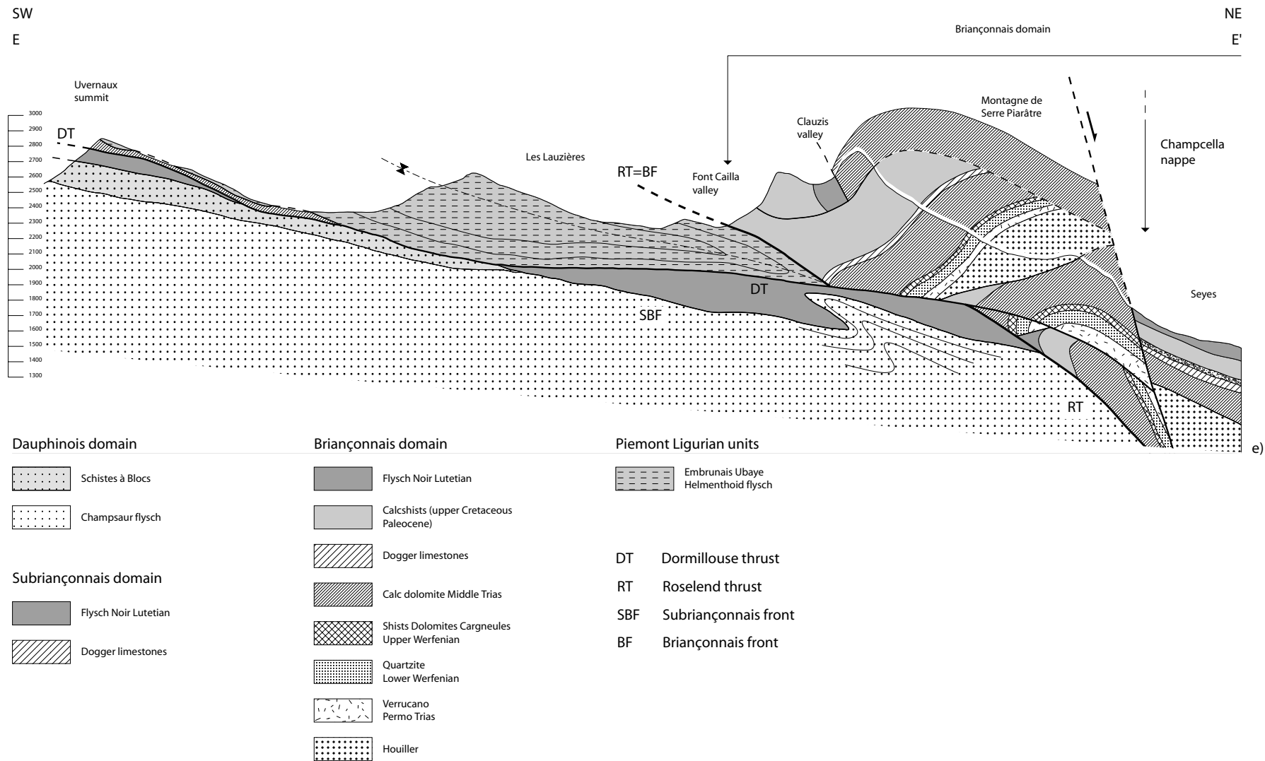
Figure 1.11: E-E' cross section. See profile trace on figure 1.2.
