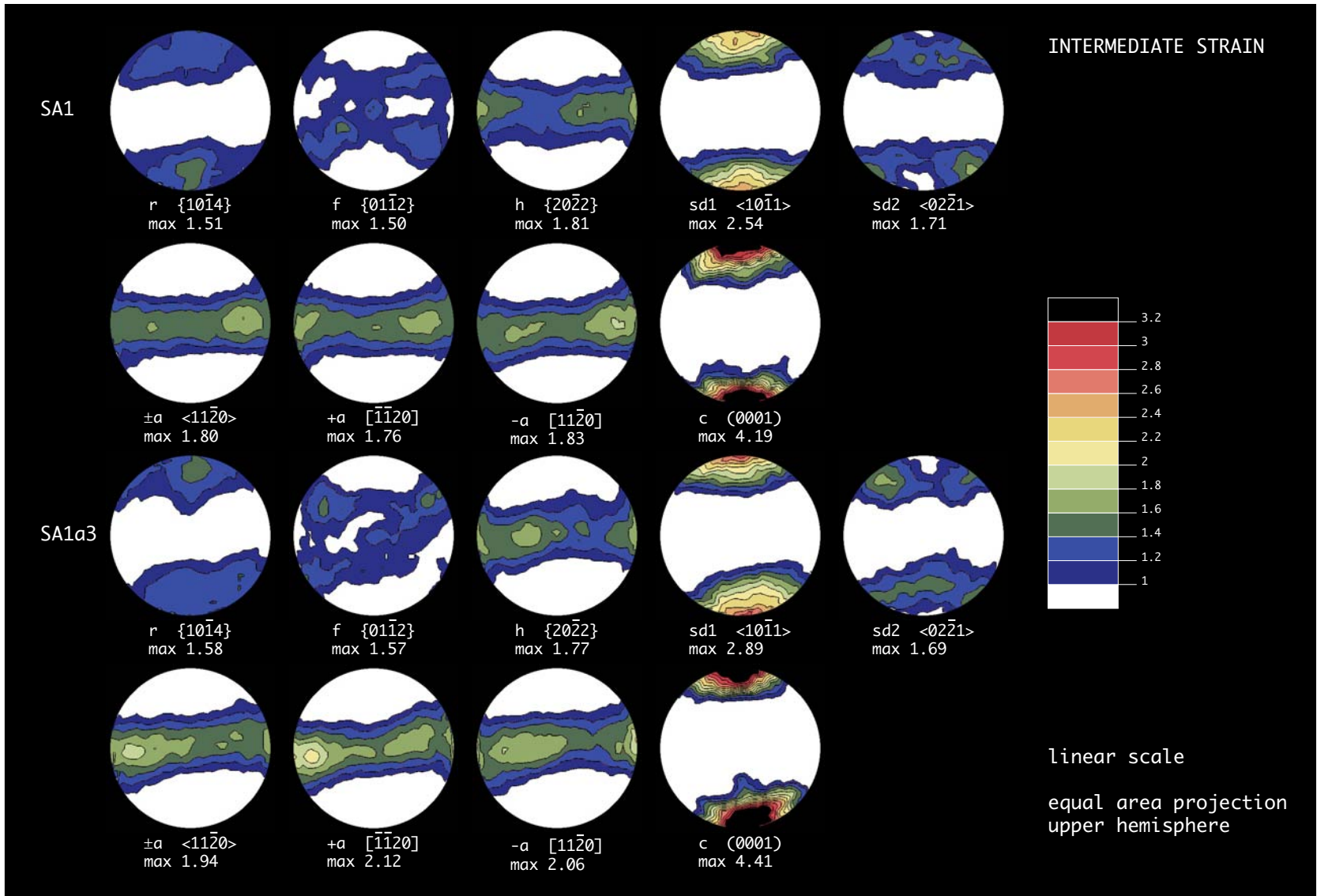
Figure B19: Crystallographic preferred orientation of samples SA1 and SA1a3.
