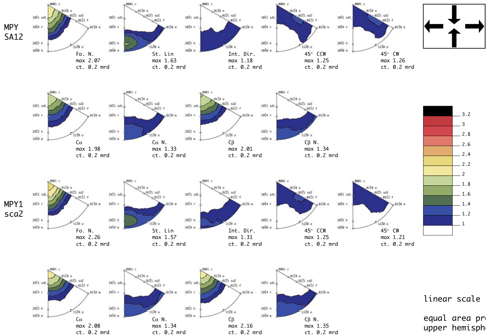
Figure B24: Inverse pole figures calculations for samples MPYSA12 and MPY1sca2.
