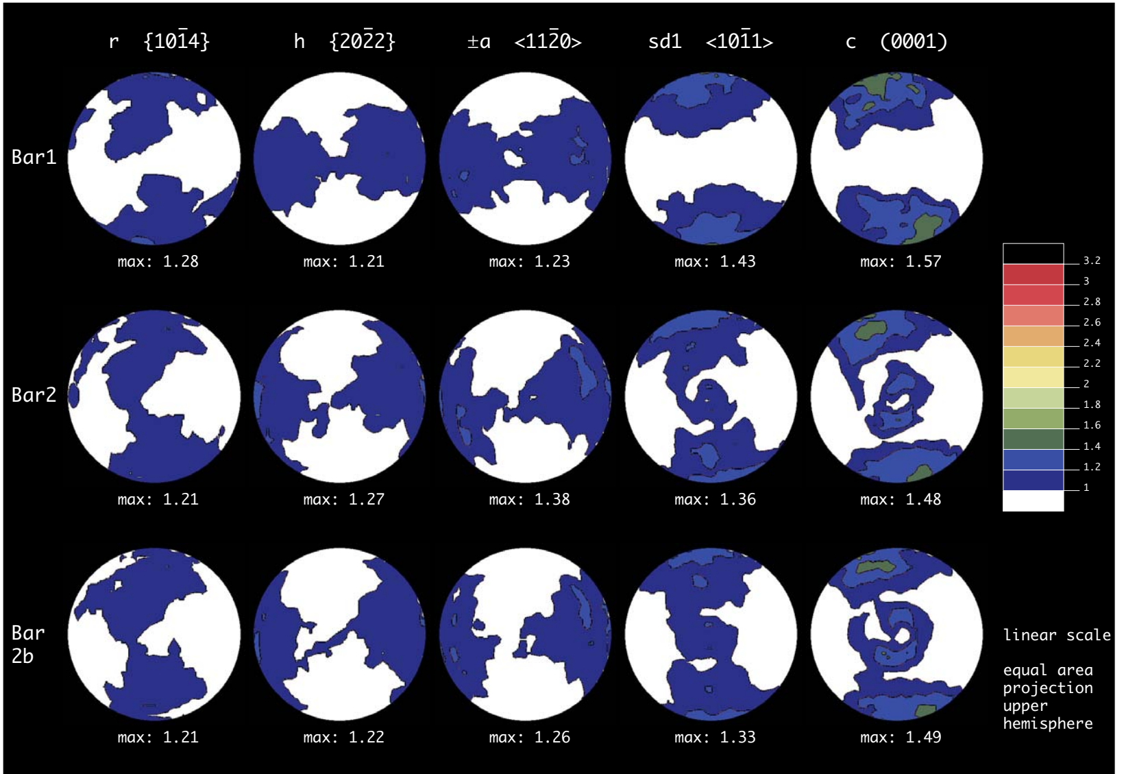
Figure 3.19a: Texture analysis of samples Bar1, Bar2 and Bar2b.
