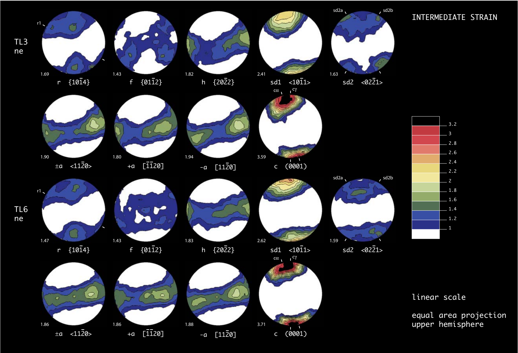
Figure 3.11: Complete texture analysis of samples TL3ne and TL6ne. Note the slight monoclinic symmetry of the texture.
