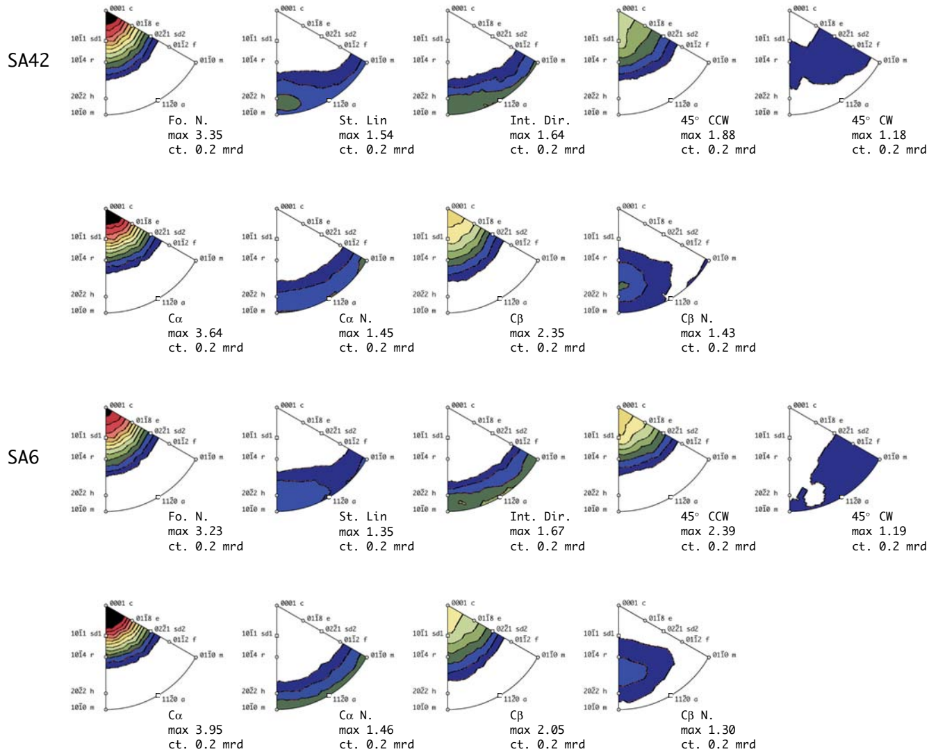
Figure B29: Inverse pole figures calculations for samples SA42 and SA6.
