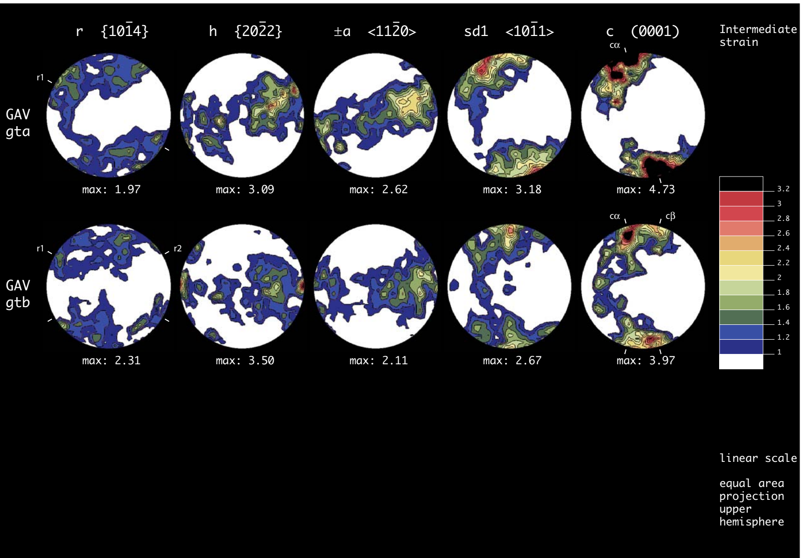
Figure 3.38: Texture analysis of samples GAVgta and GAVgtb. All pole figures show departure from orthorhombic symmetry. See text for discussion.
