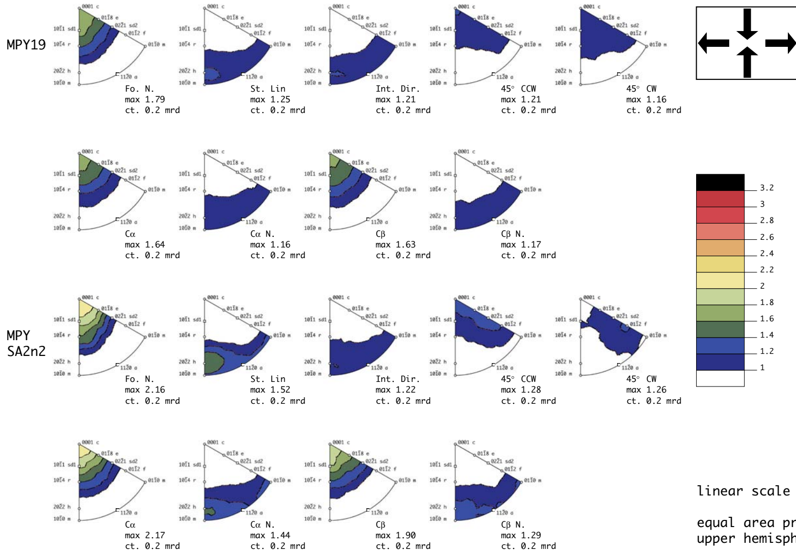
Figure B23: Inverse pole figures calculations for samples MPY19 and MPYSA2n2.
