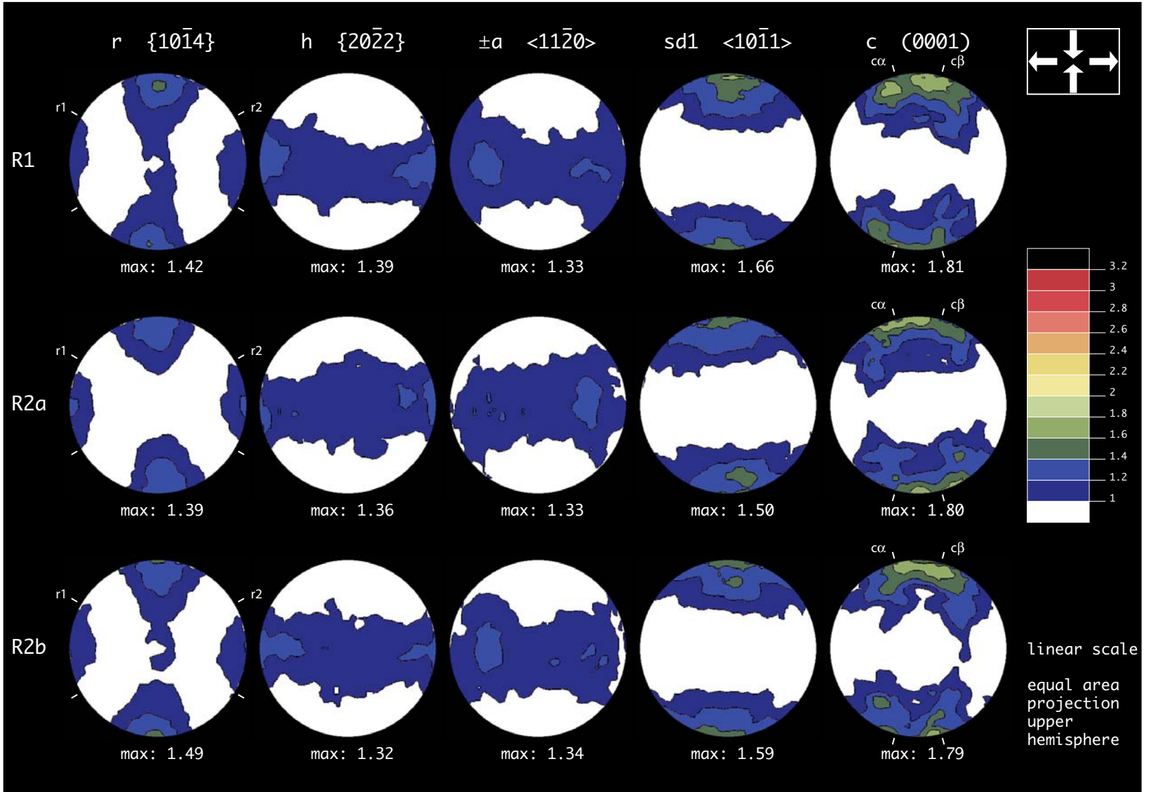
Figure 3.21: Texture analysis of samples R1, R2a and R2b.
