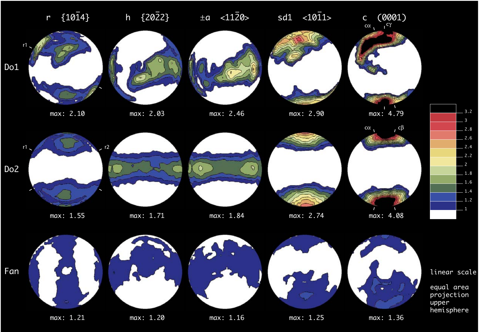
Figure 3.34: Texture analysis of samples Do1 and Do2 (Palluel lake) and Fan (Fanggas lake).
