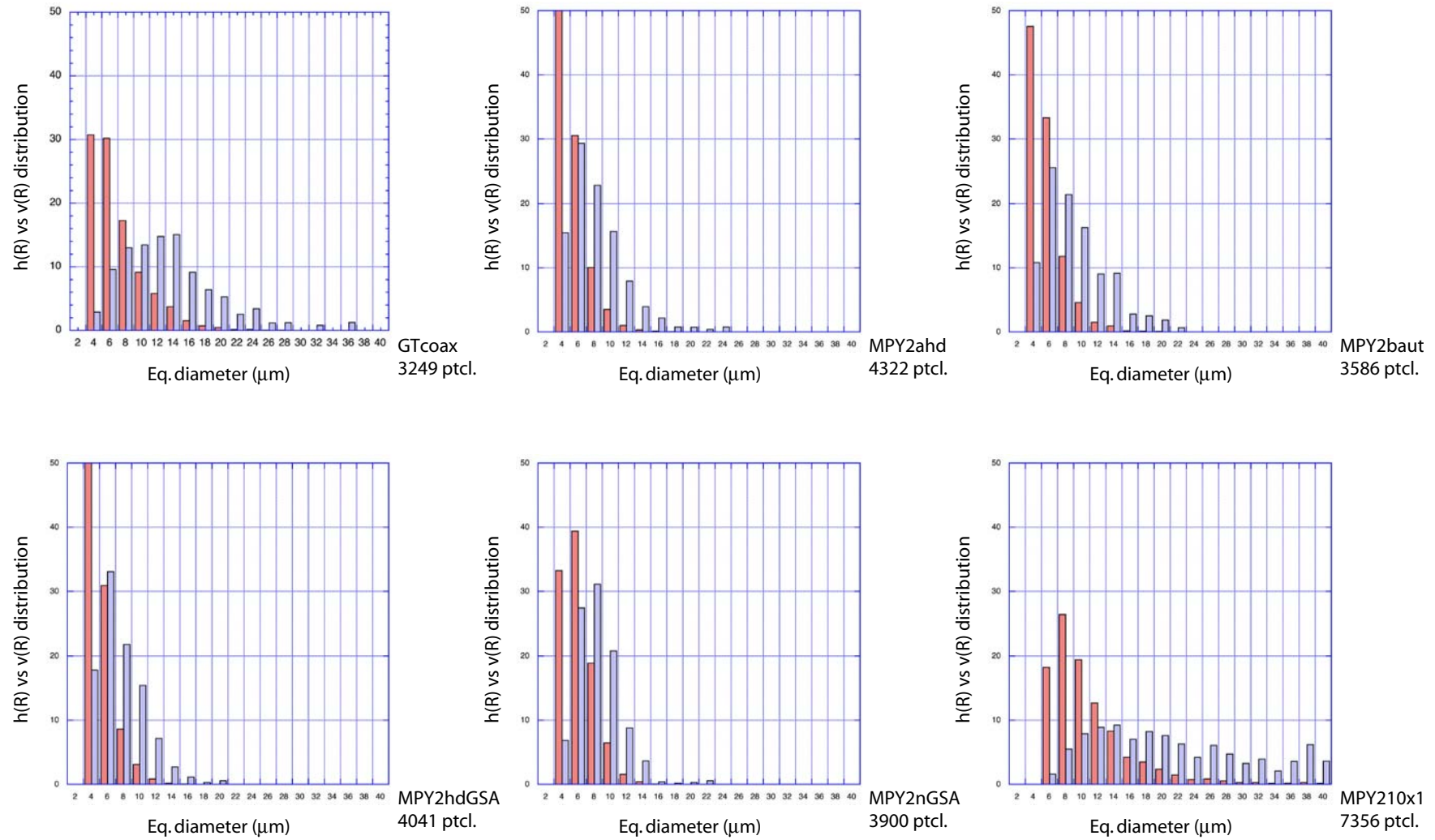
Figure B31: Grain size analysis of samples GTcoax bis MPY210x1.
