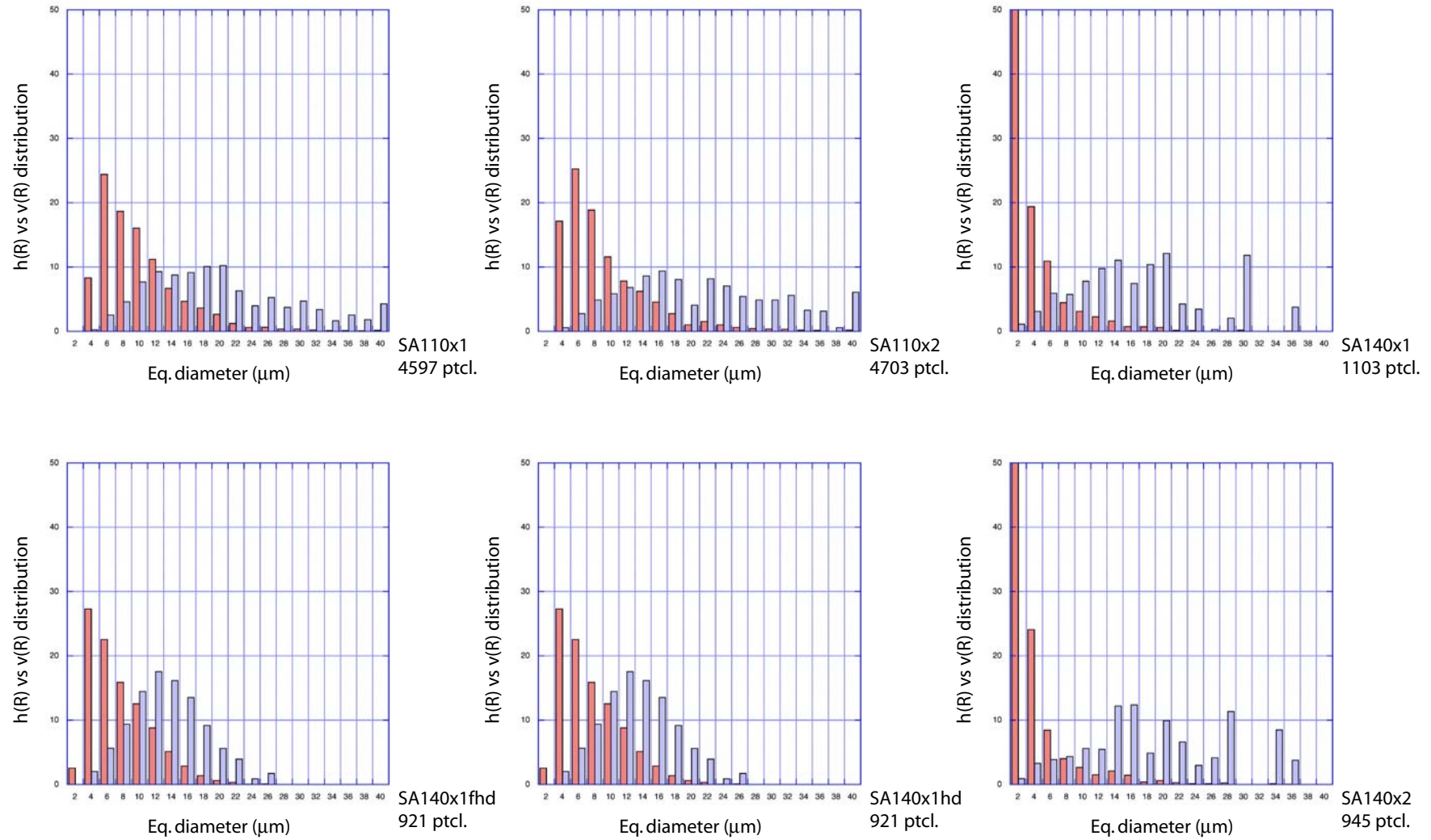
Figure B33: Grain size analysis of samples SA110x1 bis SA140x2.
