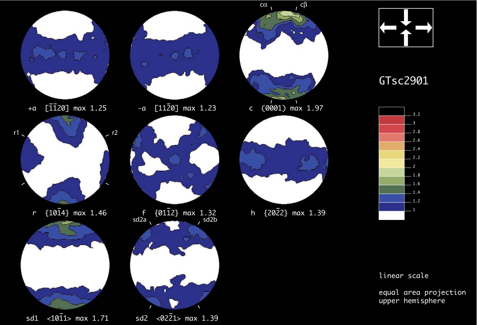
Figure 3.30: Complete texture analysis of sample Gtsc2901. Note the orthorhombic level of symmetry recorded in each pole figure.
