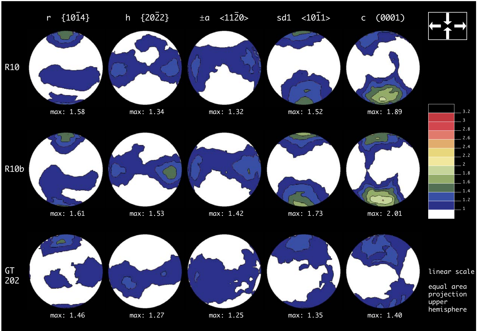
Figure 3.18b: Texture analysis of samples R10, R10b and GT202.
