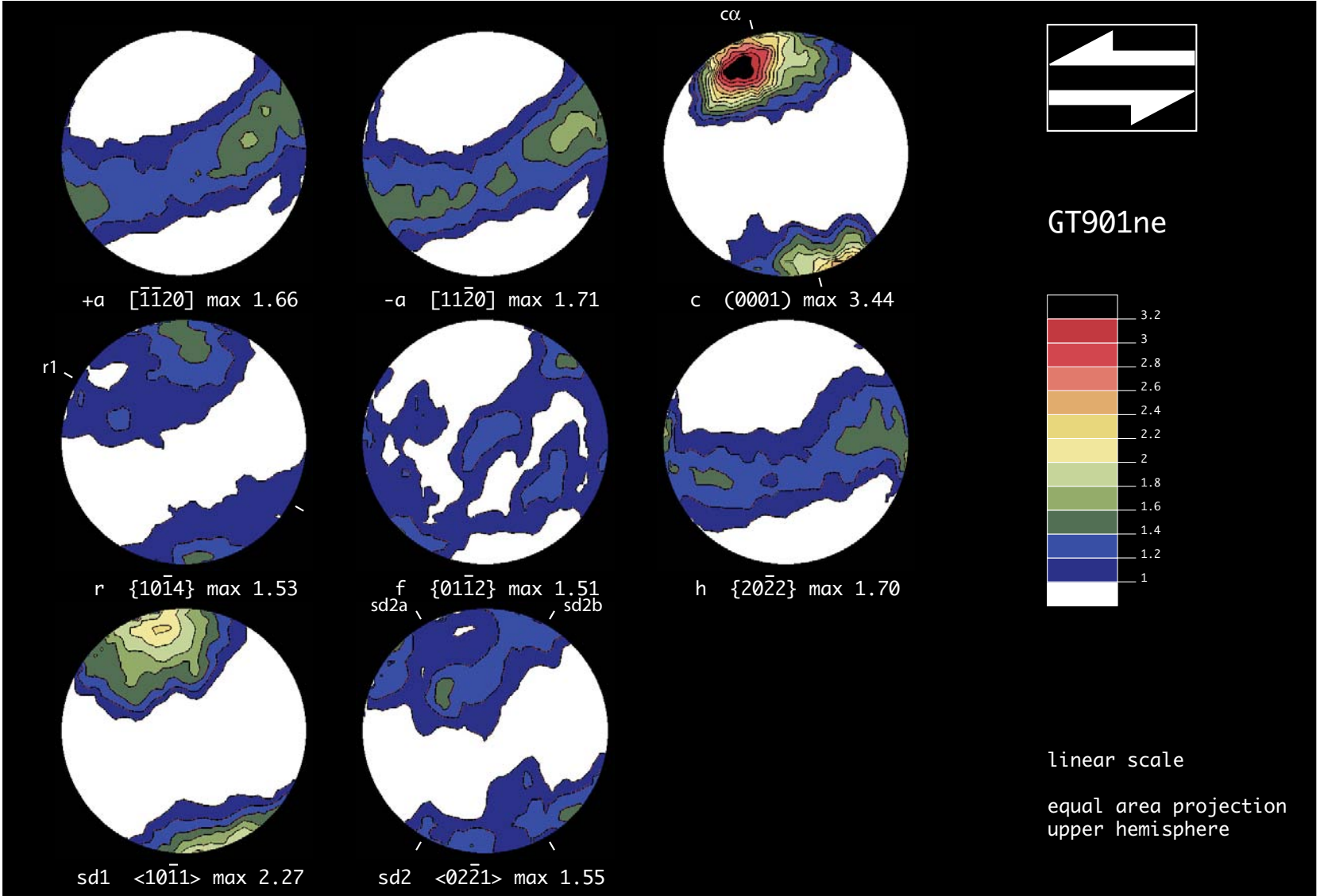
Figure 3.27: Complete texture analysis of sample GT901ne. Note the clear monoclinic symmetry of the texture developed under a non-coaxial strain path.
