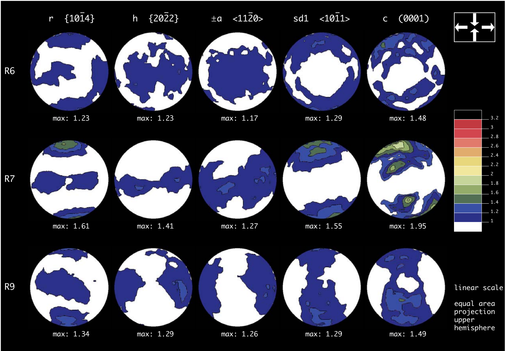
Figure 3.18a: Texture analysis of samples R6, R7 and R9.
