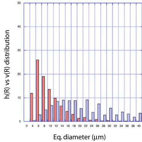
Figure B35: Grain size analysis of samples MPY22hdgsa bis GTncoax.
