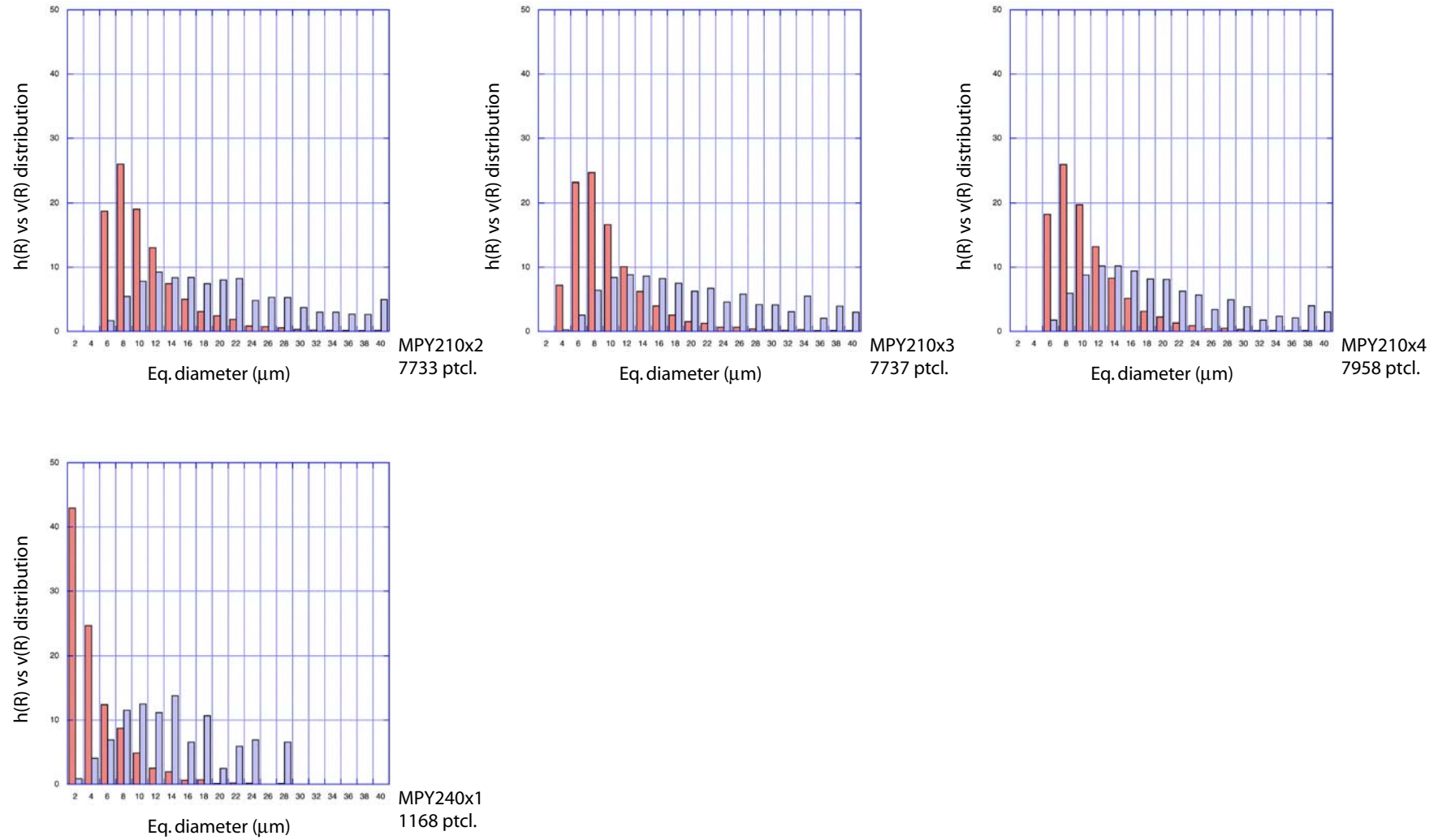
Figure B32: Grain size analysis of samples MPY210x2 bis MPY240x1.
