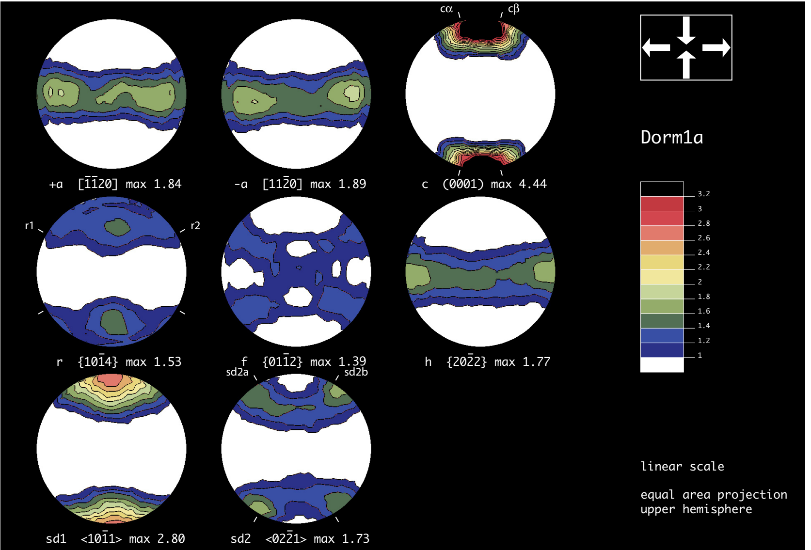
Figure 3.35: Complete texture analysis of sample Dorm1a. Note the orthorhombic level of symmetry recorded in each pole figure.
