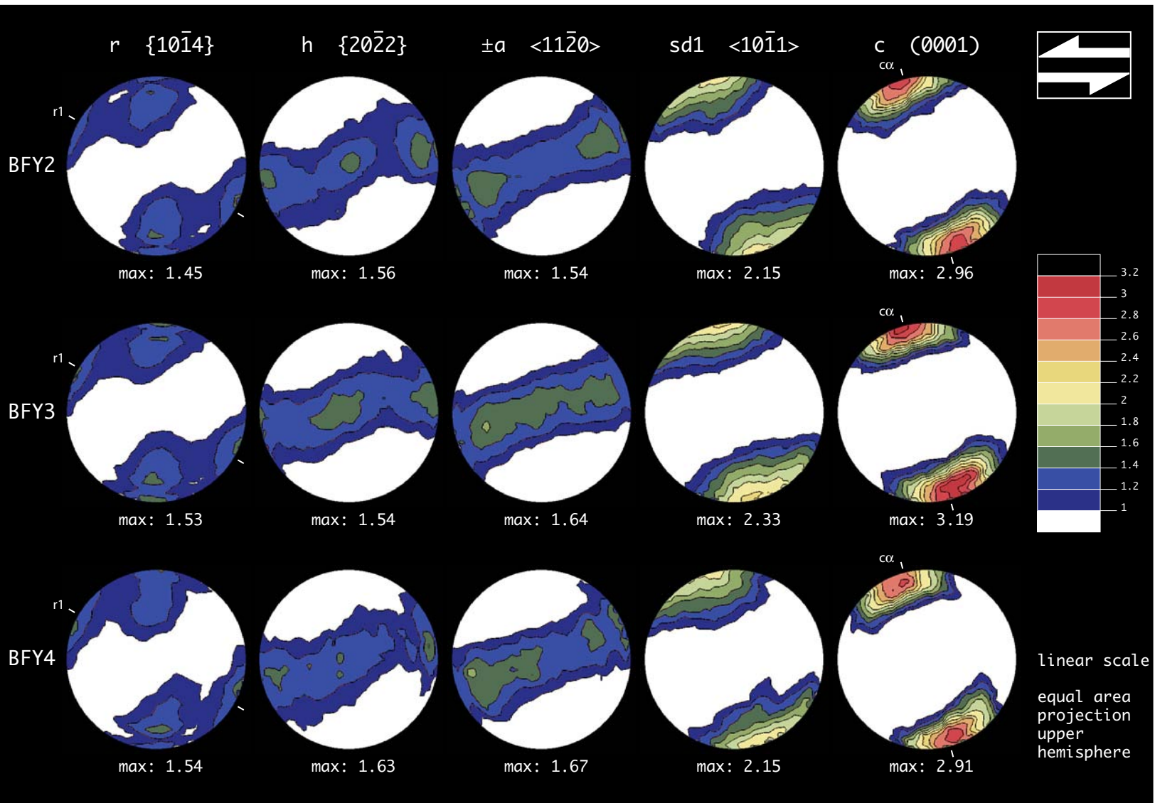
Figure 3.5: Crystallographic preferred orientation (CPO) of samples BFY2, BFY3 and BFY4. Note the clear monoclinic symmetry of the texture, indicative of sinistral simple shear deformation. See text for discussion.
