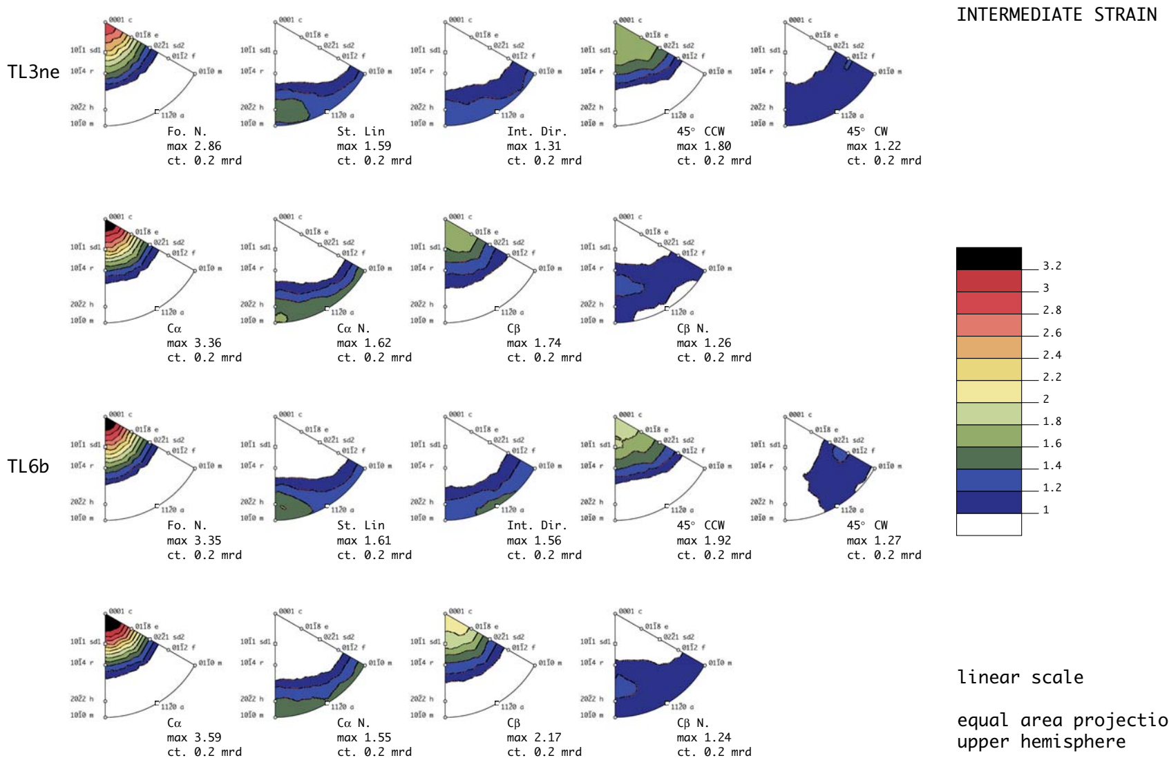
Figure 3.12: Inverse pole figures calculated for samples TL3ne and TL6b. See text for discussion.
