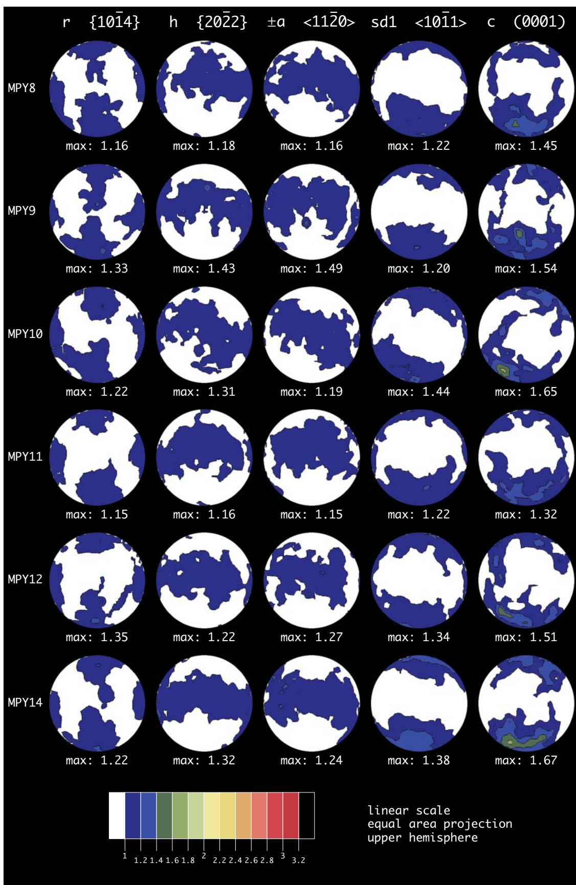
Figure B6: Crystallographic preferred orientation of samples MPY8 bis MPY14.
