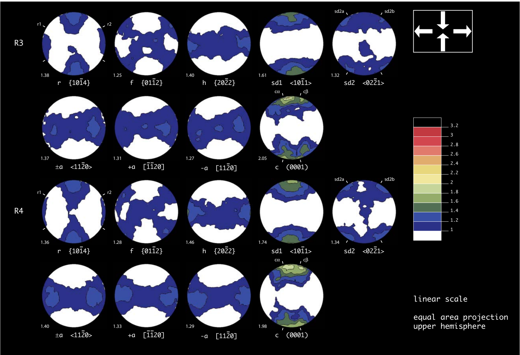
Figure 3.22: Complete texture analysis of samples R3 and R4. Note the splitting of the c -axis distribution at positions c\alpha and c\beta .
