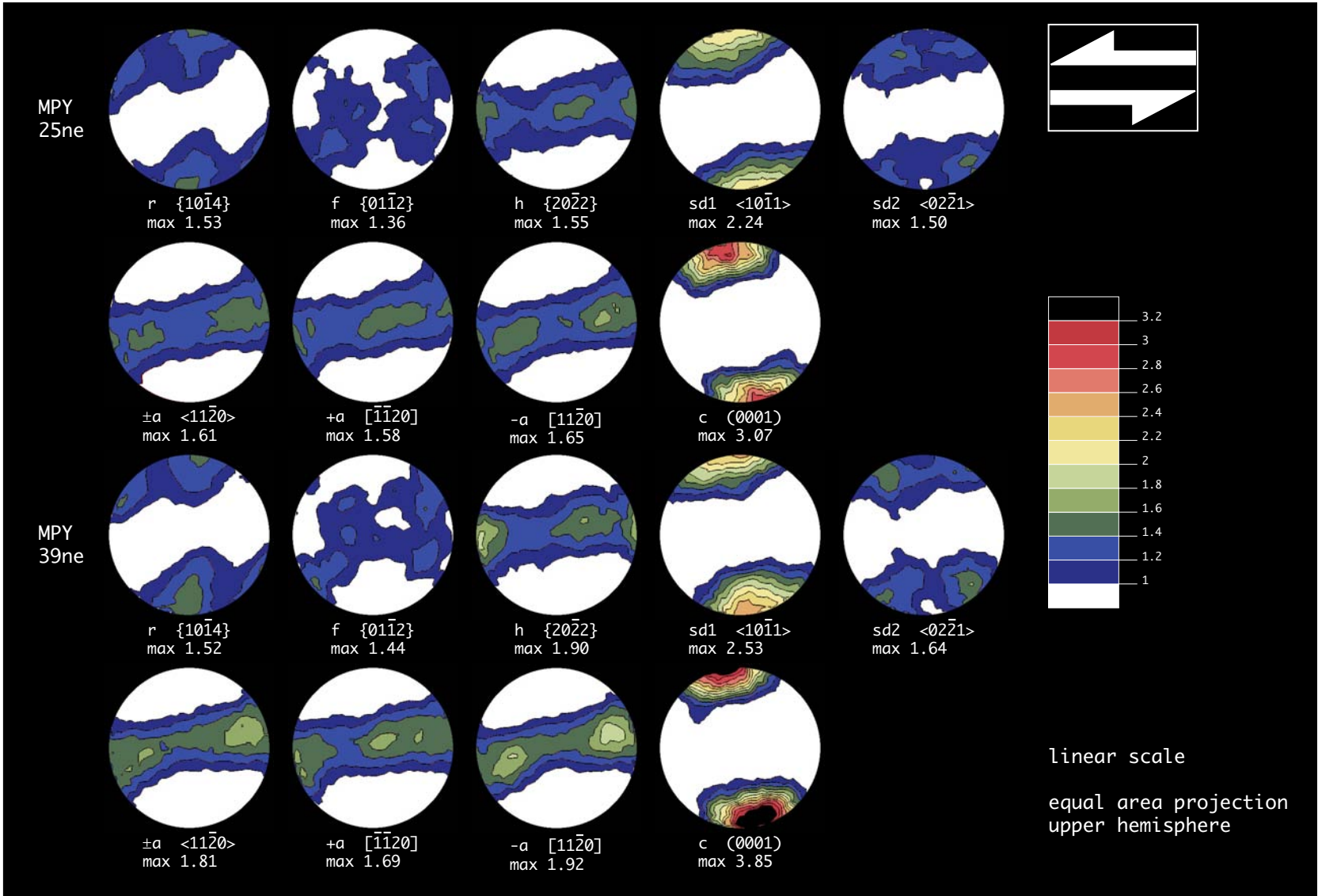
Figure B21: Crystallographic preferred orientation of samples MPY25ne and MPY39ne.
