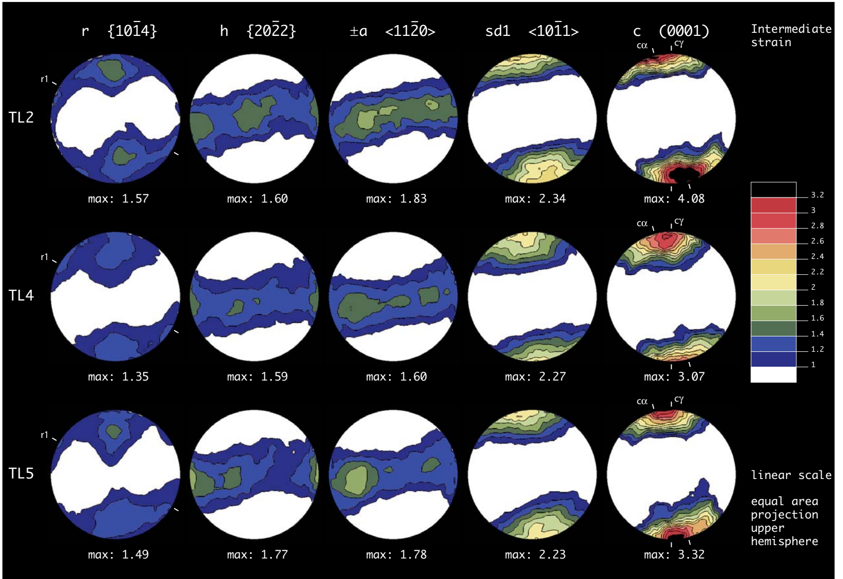
Figure 3.10: Texture analysis of samples TL2, TL4 and TL5.
