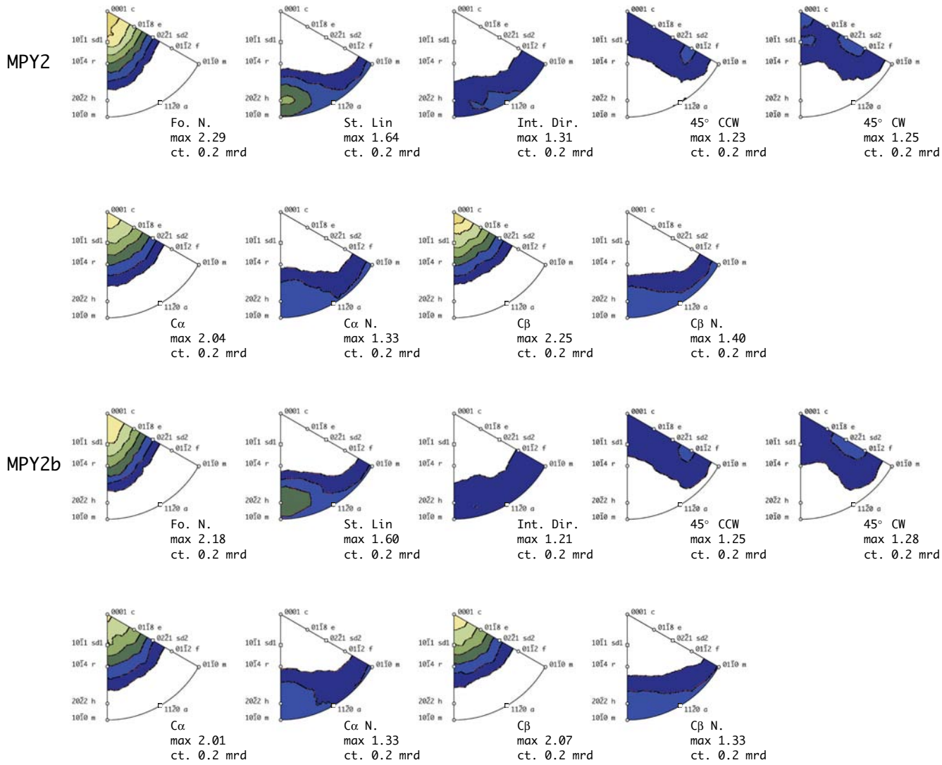
Figure B25: Inverse pole figures calculations for samples MPY2 and MPY2b.
