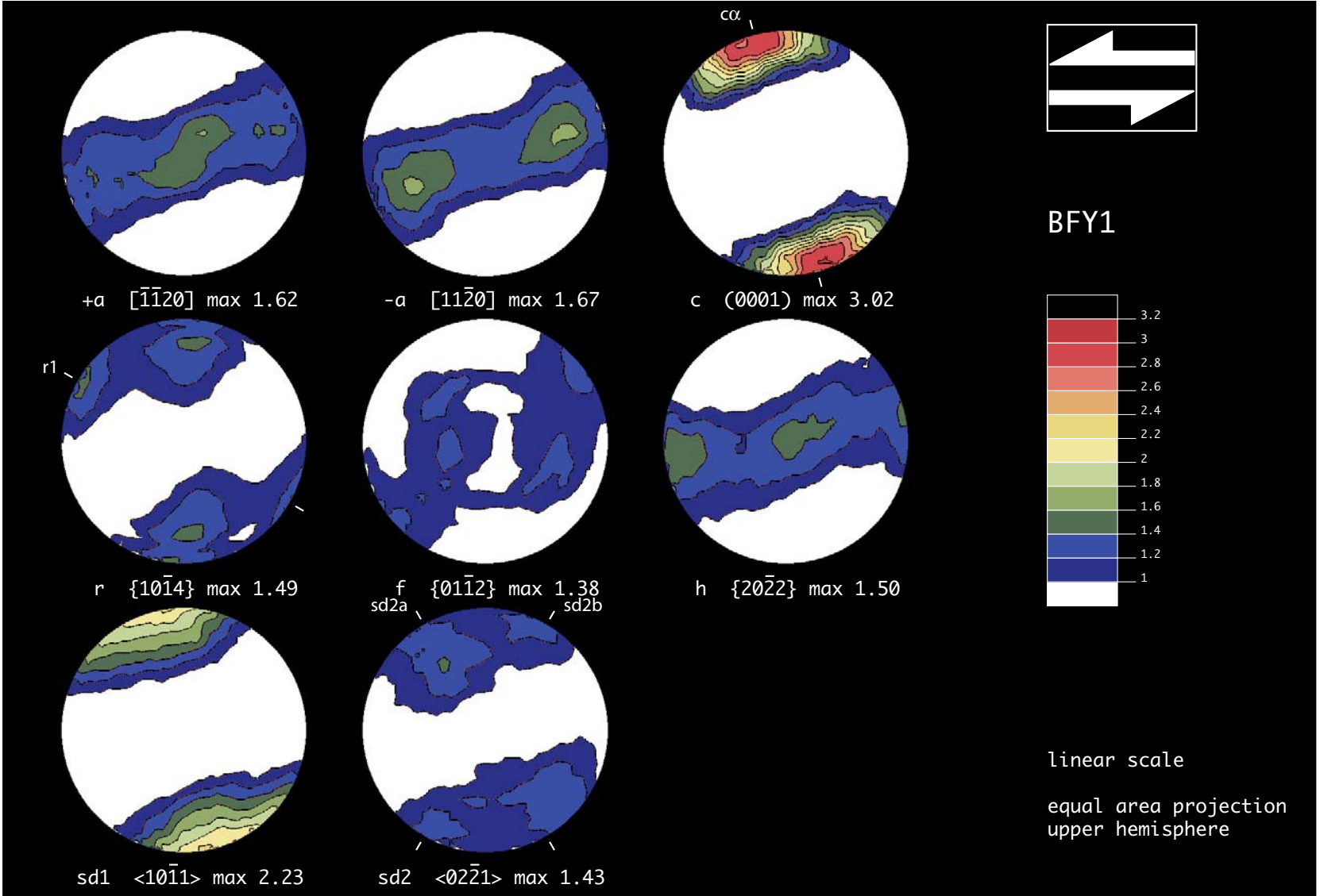
Figure 3.6: Complete texture analysis of sample BFY1. Note the different distribution of +a and -a directions on the non-reduced a pole figures.
