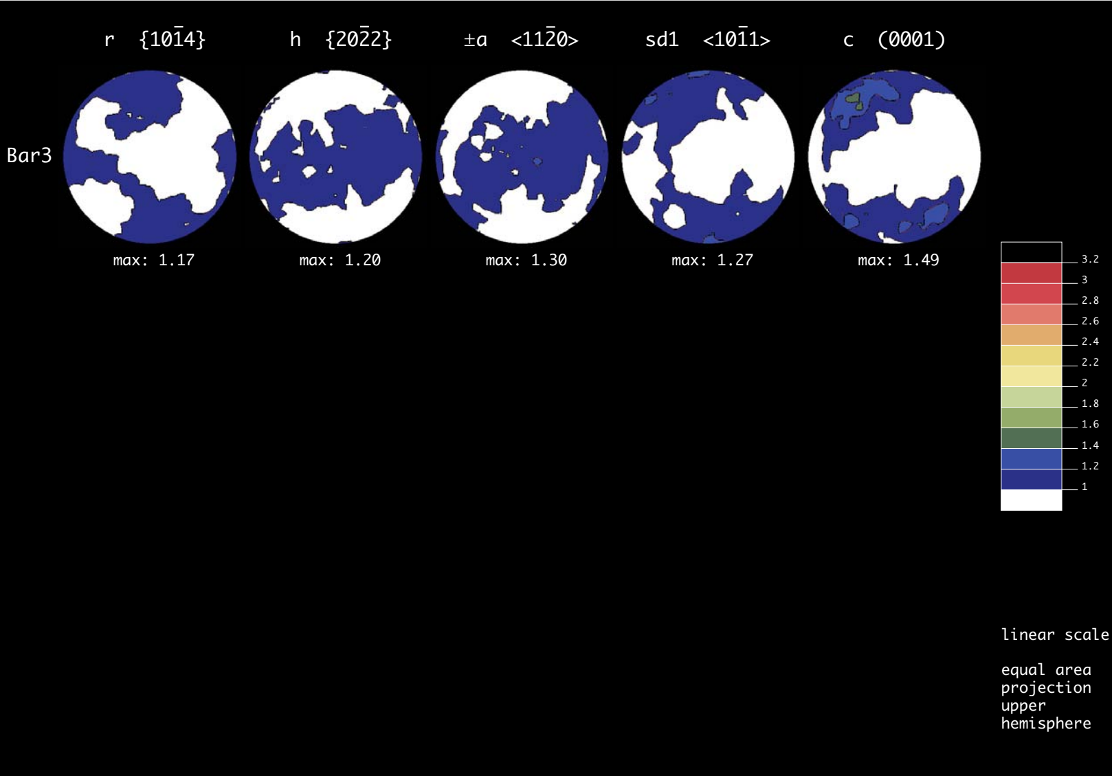
Figure 3.19b: Texture analysis of sample Bar3.
