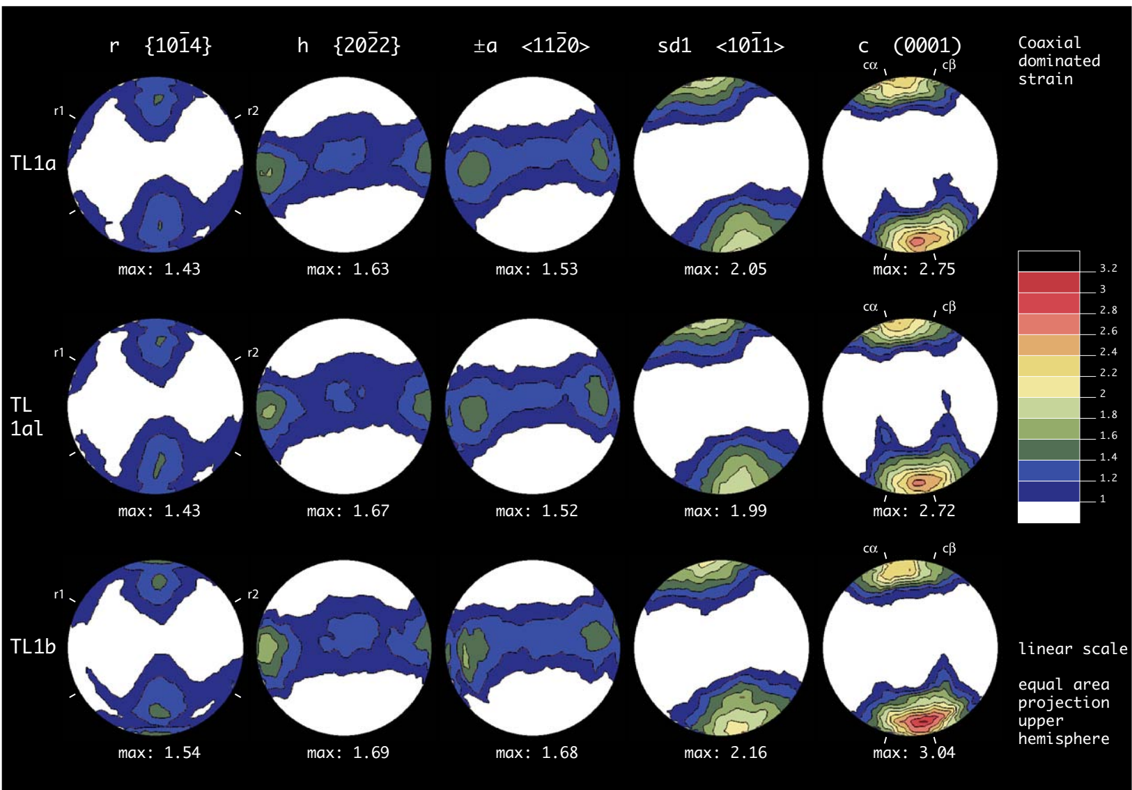
Figure 3.14: Texture analysis of samples TL1a, TL1a1 and TL1b. Note the nearly orthorhombic level of symmetry recorded by each pole figure.
