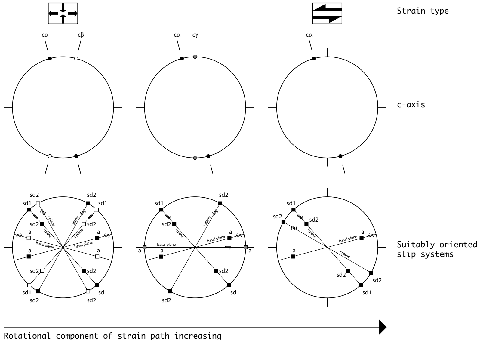
Figure 2.18: Sketch summarizing the evolution of the calcite c -axis distribution during the transition from coaxial dominated to non-coaxial dominated deformation under conditions suppressing twinning. Poles and projections of slip planes and slip directions are reported for the main ideal orientation components, which are suitably oriented for slip under the assumed kinematics. Black symbols belong to orientations with c -axis at c\alpha (M1, M3), white symbols at c\beta (M2), grey symbols at c\gamma (M4, M4').
