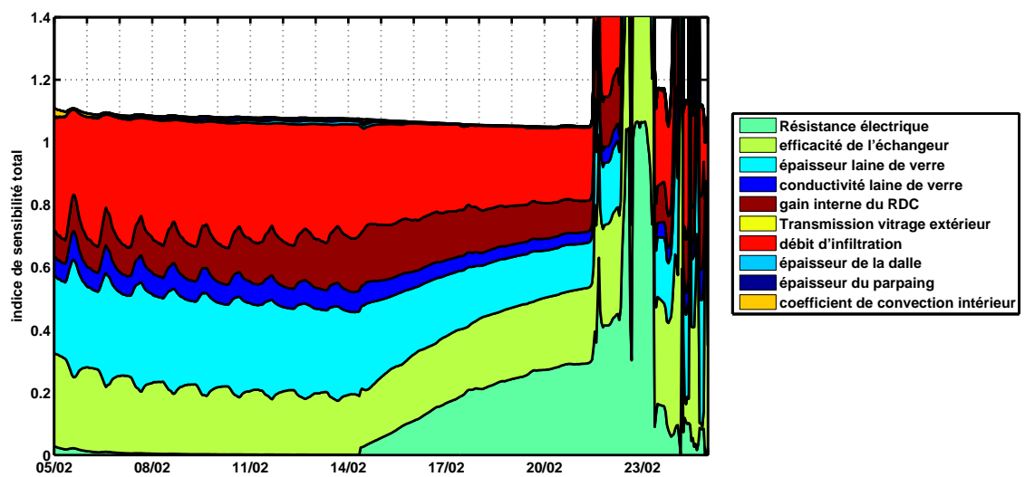
(b) Indice total
