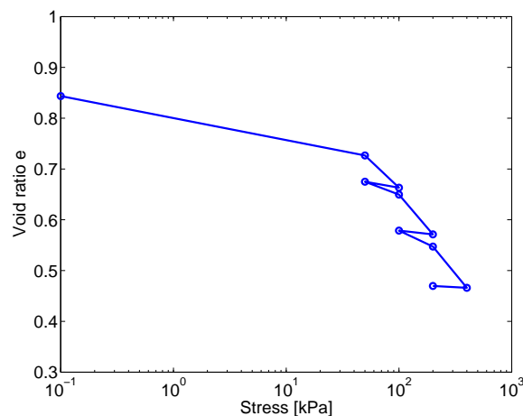
Figure 3.13: Isotropic compression stress-strain path
