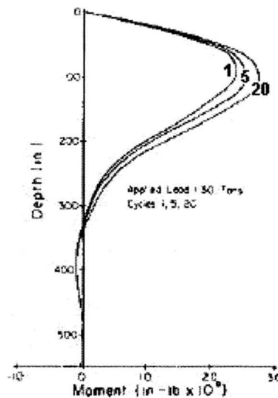
Figure 2.30: Bending moment evolution with cyclic lading (Reese and Welch, 1975)
