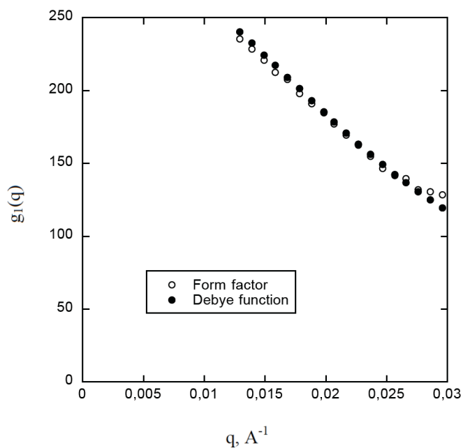
Figure 18. Fit of g_1(q) with g_D(q) for PSS ( N = 300 ) solutions in IL2 (SANS).
