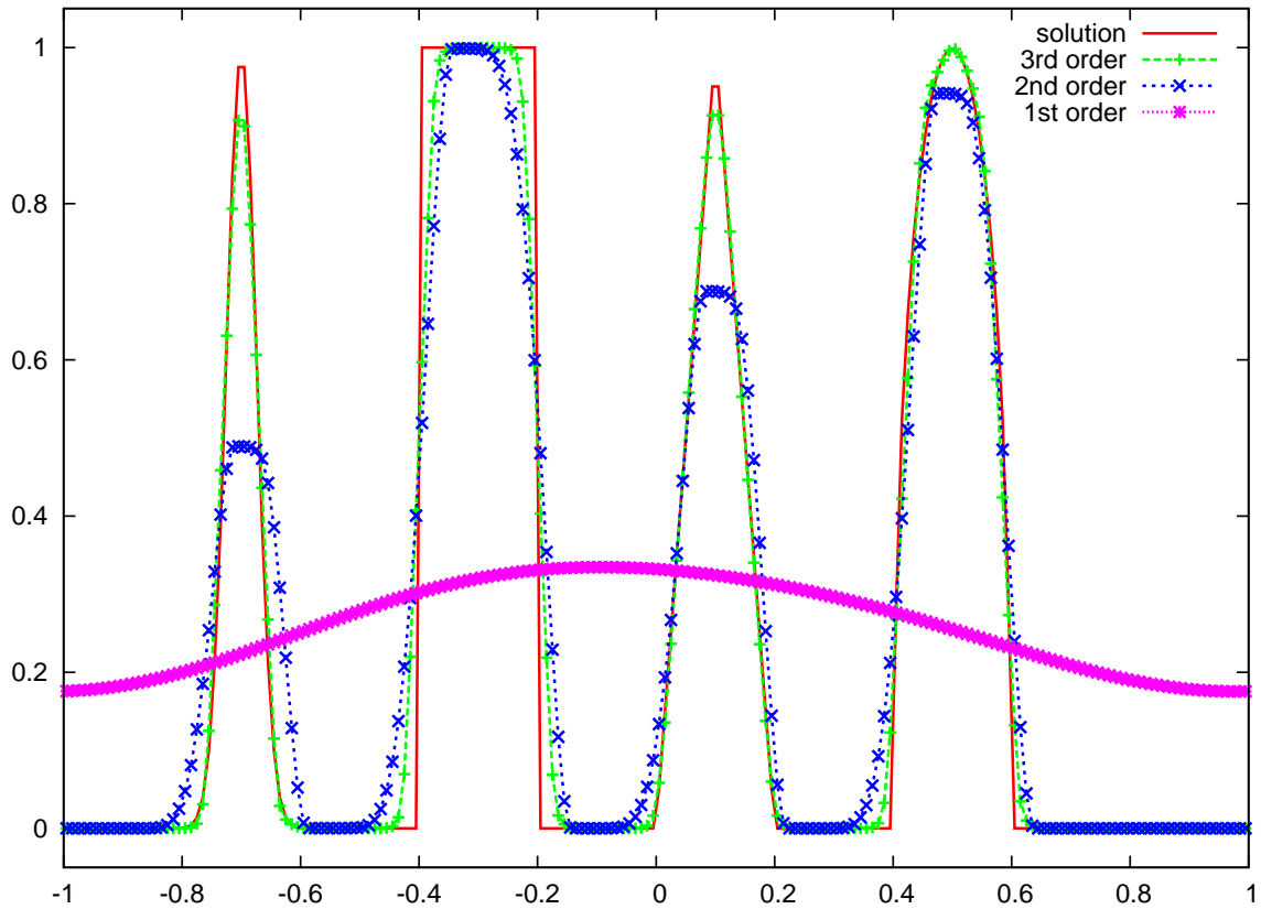
Figure 1.14: Linear advection ( a = 1 ) of the composite signal (1.58), with periodic boundary conditions, at the end of ten periods with a CFL=0.2 and on [-1, 1] with a grid characterized by 200 uniformly spaced cells. Comparison between the analytical solution and the numerical solutions obtained with the first, second and third-order DG schemes with the hierarchical vertex-based slope limiter.
