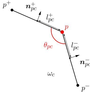
Figure 3.8: Corner angle of a polygonal cell.
