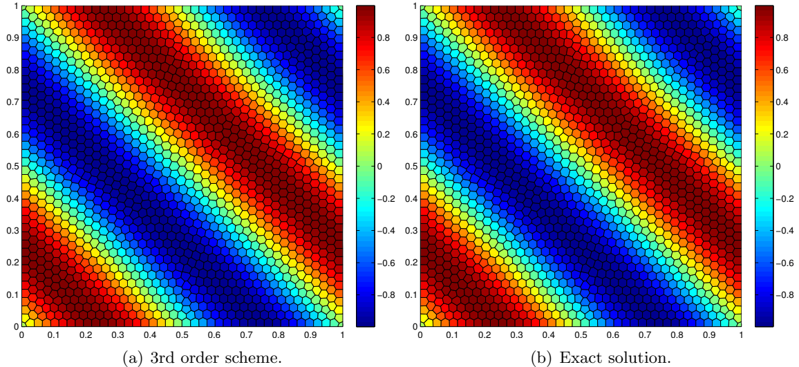
Figure 1.28: Linear advection ( \mathbf{A} = (1, 1)^\dagger ) of the smooth initial condition u^0(\mathbf{x}) = \sin(2\pi(x+y)) where \mathbf{x} = (x, y)^\dagger \in [0, 1]^2 , with periodic boundary condition, at the end of a period on an unstructured grid made of 1600 polygonal cells.
