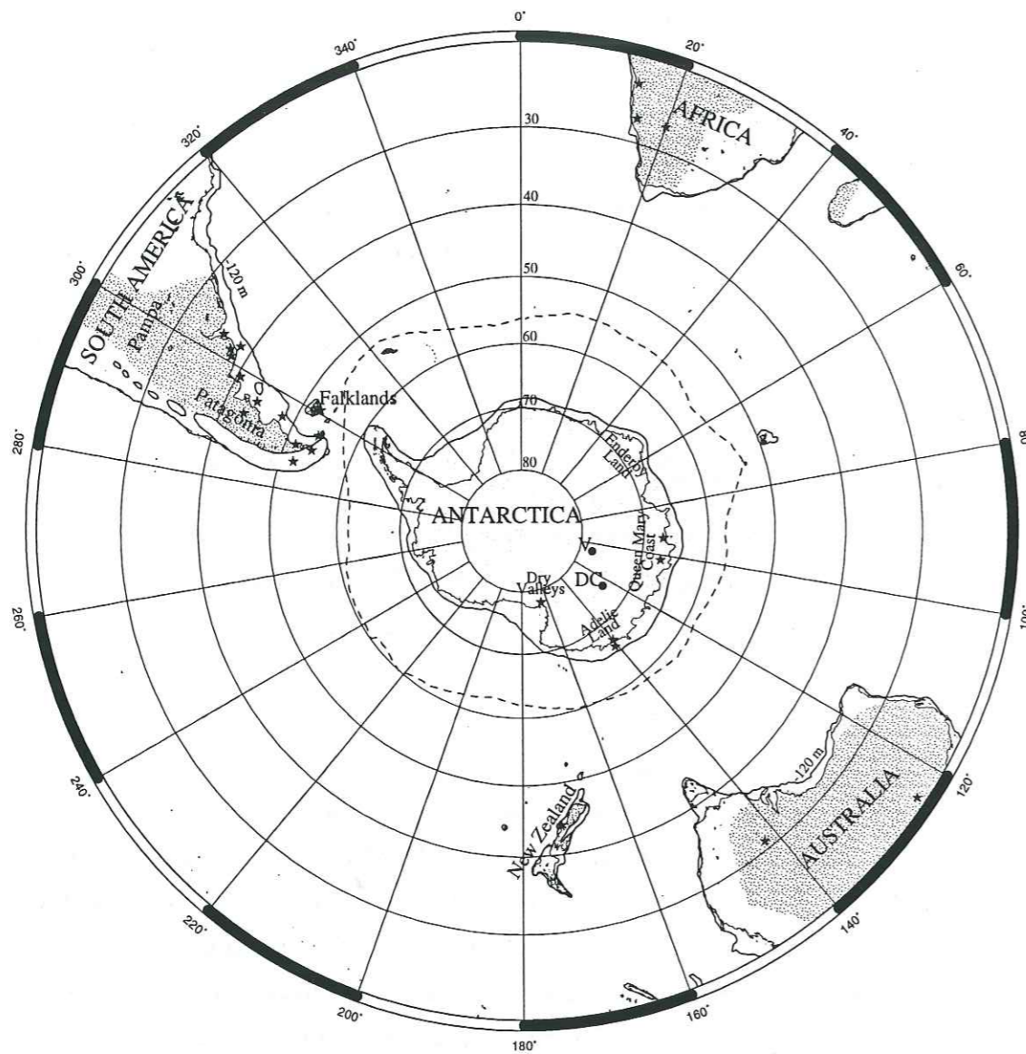
Figure 4-9 : Schematic polar projection of the Southern Hemisphere during the LGM. Grey areas represent ice cape extensions over the Andes, the New Zealand Alps and Antarctica (Broecker and Denton, 1990 ; Clapperton, 1993). Dashed line represents the supposed sea-ice extension around Antarctica (Clapperton, 1993). Stippled areas represent arid and desertic regions (adapted from Bowler, 1976 ; Clapperton, 1993 ; McGinnies, 1968). The isobath at -120 m shows the maximum extension of the exposed continental shelves. Stars show the sampling location of sources samples. V = Vostok drilling site. DC = Dome C drilling site.
