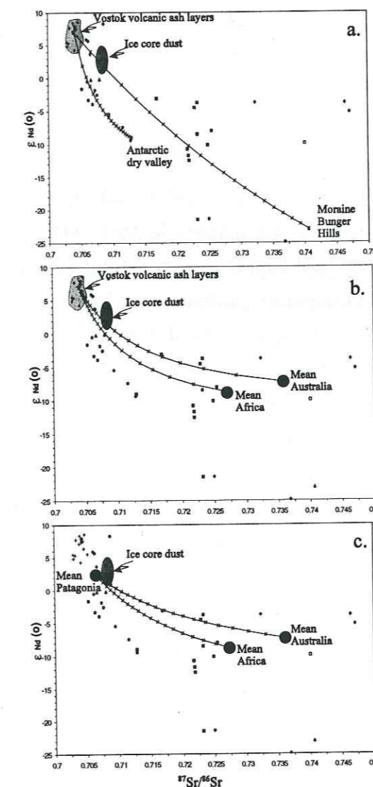
Figure 4-13 : Theoretical mixing hyperbolae constructed on a \epsilon_{\text{Nd}} (‰) versus ^{87}\text{Sr}/^{86}\text{Sr} . (Same symbols as on Figure 4-11). Hyperbolae are for mixing curves between two end members. The graduations on the mixing hyperbolae occur every 5% (Taylor and McLennan, 1985). (a) Hypothesis 1 with two local Antarctic end-members ; (b) Hypothesis 2 with a local volcanic end-member plus a remote continental end-member ; (c) Hypothesis 3 with Patagonia and a remote desertic end-member.
