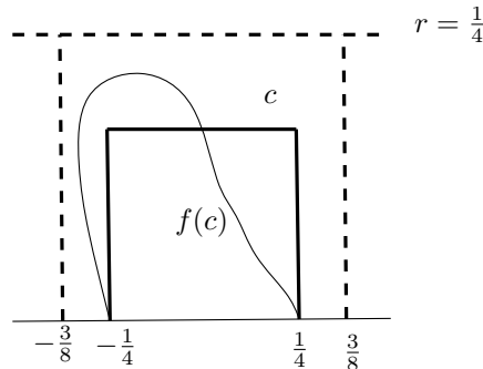
Figure 4.2: Description of the curve c
