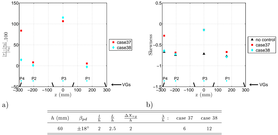
Figure 4.19: a) Gain in friction and b) Skewness for cases 37 and 38 (i.e. for two different values of \frac{\lambda}{h} and the other parameters kept constant).
