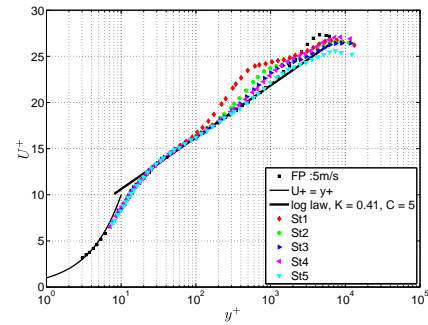
Figure 6. Mean velocity profiles, \alpha = -2^\circ , \beta = -22^\circ and U_\infty = 10 m/s.
