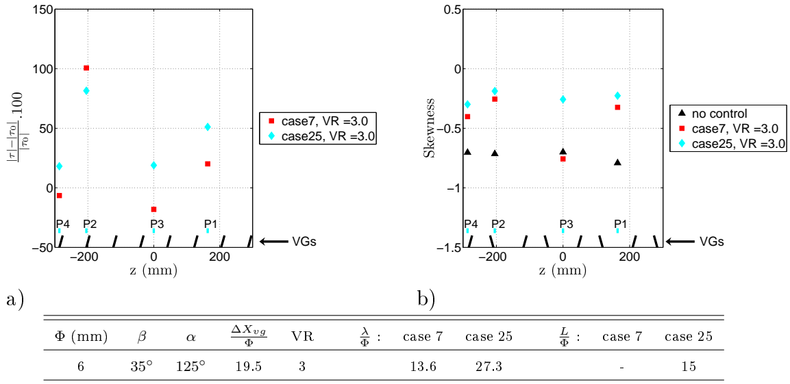
Figure 5.41: a) Gain in friction and b) Skewness for cases 7 (co-rotating configuration) and 25 (counter-rotating configuration), VR = 3 (i.e. for co and counter-rotating VGs configurations with similar parameters).
