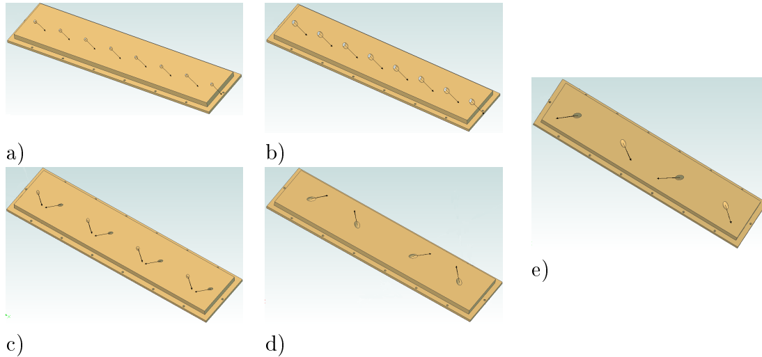
Figure 2.3: Insert for a) co-rotating \Phi = 6 mm, b) co-rotating \Phi = 12 mm, c) counter-rotating \Phi = 6 mm, d) counter-rotating \Phi = 12 mm and \frac{L}{\Phi} = 15 , e) counter-rotating \Phi = 12 mm and \frac{L}{\Phi} = 12.3 .
