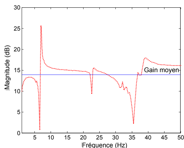
Figure 4.23 Fonction de transfert G(s) (force/tension).
