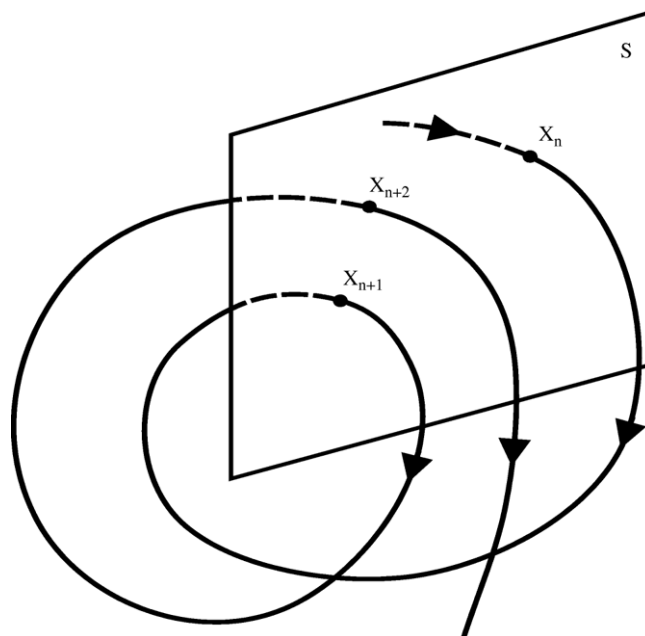
Figure 2.7 Poincaré map.
