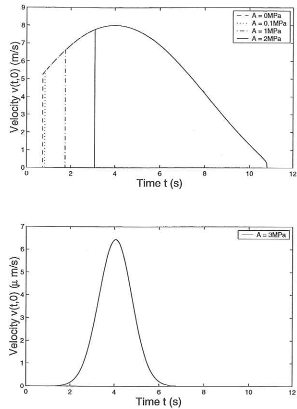
FIG. 1.17 – The effect of A in the Perrin et al. model in the context of the slab. One observes that A has a delaying effect for the instability. On the bottom figure, we see that large values of A may inhibit the instability phenomenon in the case of cycles of load. The numerical values are \mu = 34.3\text{GPa} , \rho = 2800\text{kg}\cdot\text{m}^{-3} , V_0 = 1.0 \cdot 10^{-9}\text{m}\cdot\text{s}^{-1} , V_\infty = 1.0 \cdot 10^9\text{m}\cdot\text{s}^{-1} , \tau_s = 100\text{MPa} , B - A = 2.3\text{MPa} , L = 0.1\text{mm} , \tau_0^0 = 0.9\tau_s , \tau^0 = 0.36\tau_s and T_{load} = 8\text{s} .
