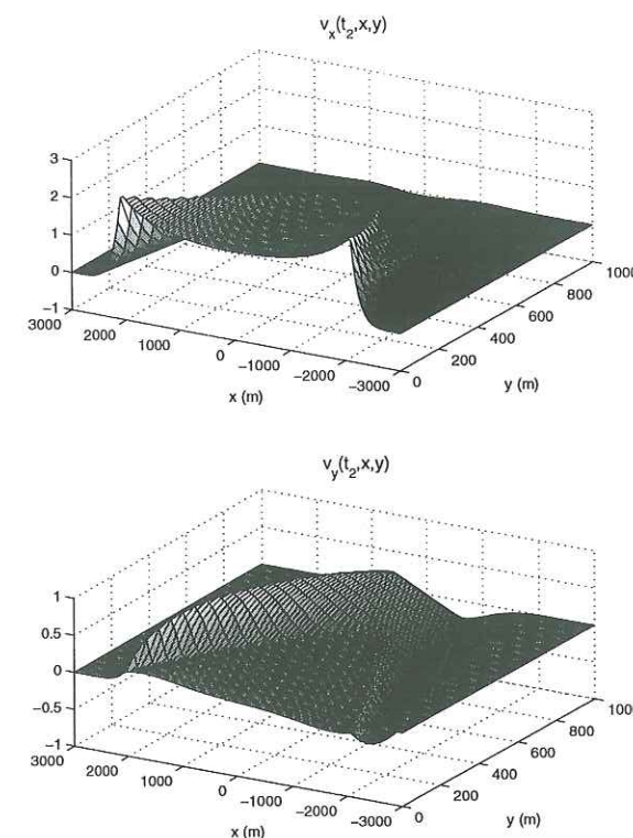
FIG. 2.14 – The plot of the velocities at t_2 = 0.5882s in the propagation phase. Here the two traveling wave front of P and S waves are visible.
