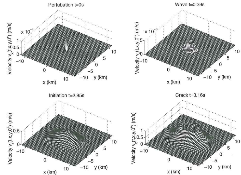
FIG. 3.3 – The process of initiation for an infinite fault. Numerical Values are \rho = 3000 \text{kgm}^{-3} , v_s = 3333 \text{ms}^{-1} , \eta = v_p/v_s = \sqrt{3} , \sigma_s - \sigma_d = 10 \text{MPa} , L_c = 0.18 \text{m} .
