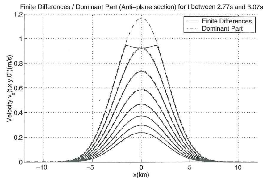
FIG. 3.5 – Numerical test of the dominant part. Numerical Values are \rho = 3000 \text{kgm}^{-3} , v_s = 3333 \text{ms}^{-1} , \eta = v_p/v_s = \sqrt{3} , \sigma_s - \sigma_d = 10 \text{MPa} , L_c = 0.18 \text{m} .
