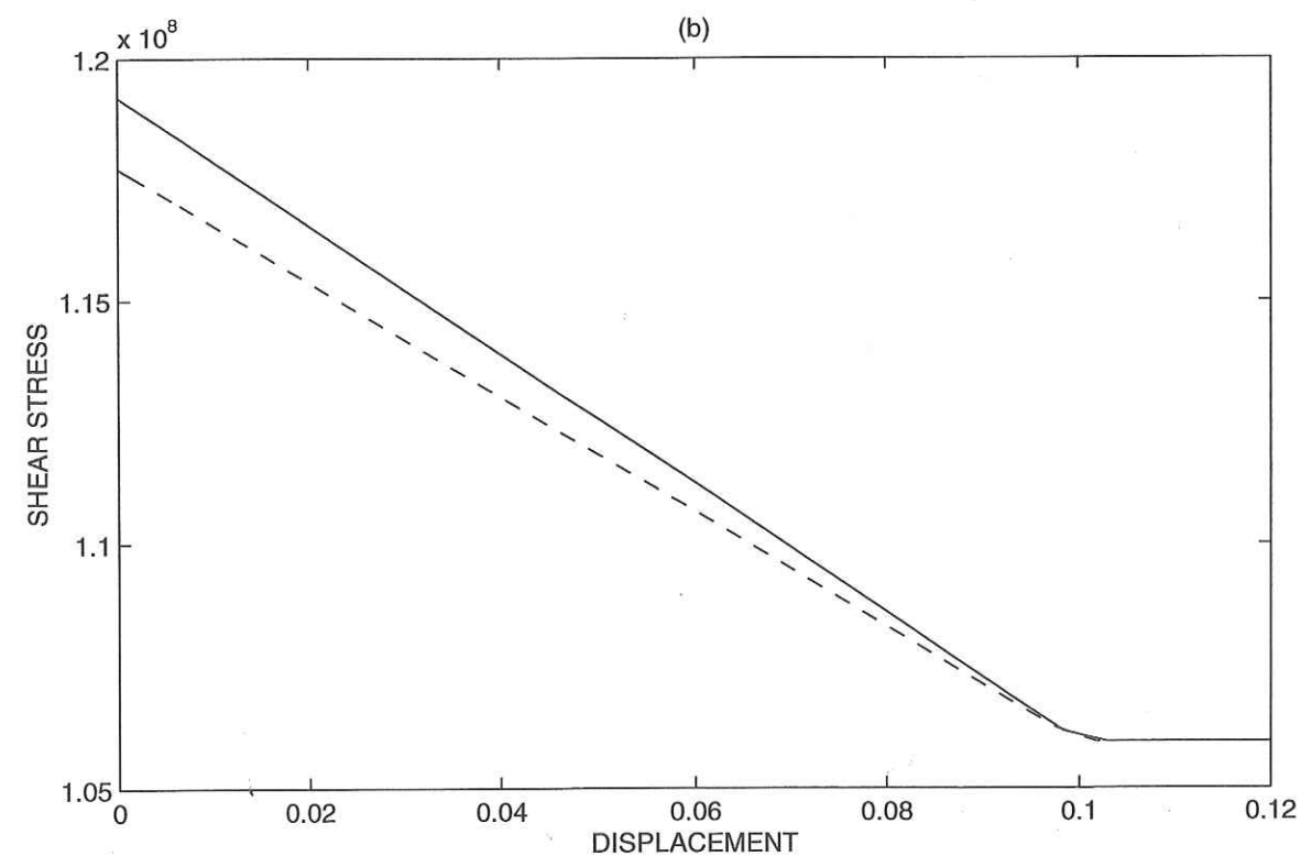
FIG. 4.1 - a) Static friction coefficient on the fault. The extremities are assumed to be unbreakable. b) The friction law on the strong (continuous line) and weak (dashed line) patches.
