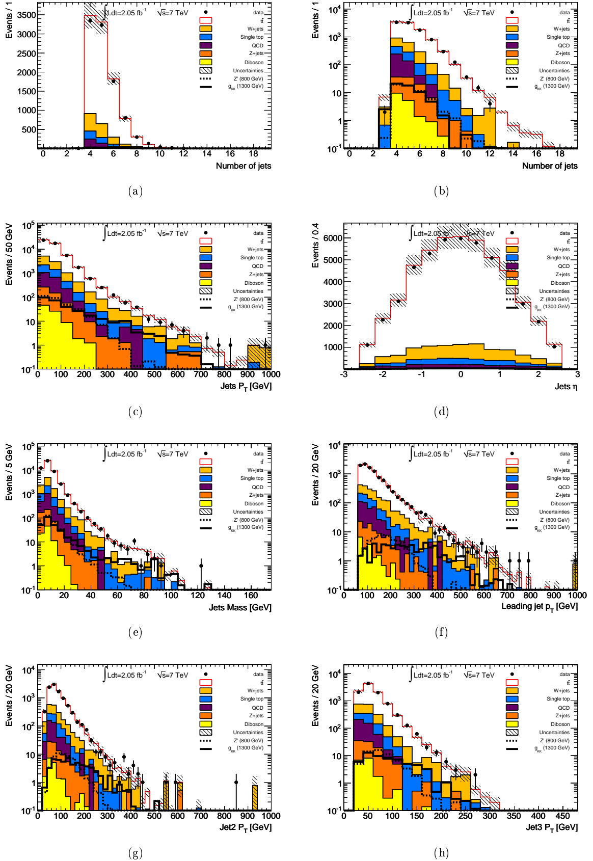
Figure D.2: Number of jets with p_T > 20 GeV in (a) linear and (b) logarithmic scales, jets (c) p_T , (d) \eta and (e) mass distributions, (f) leading jet p_T , (g) second jet p_T and (h) third jet p_T after all selection criteria were applied in the electron channel. The grey hashed area shows the total background normalization uncertainty.
