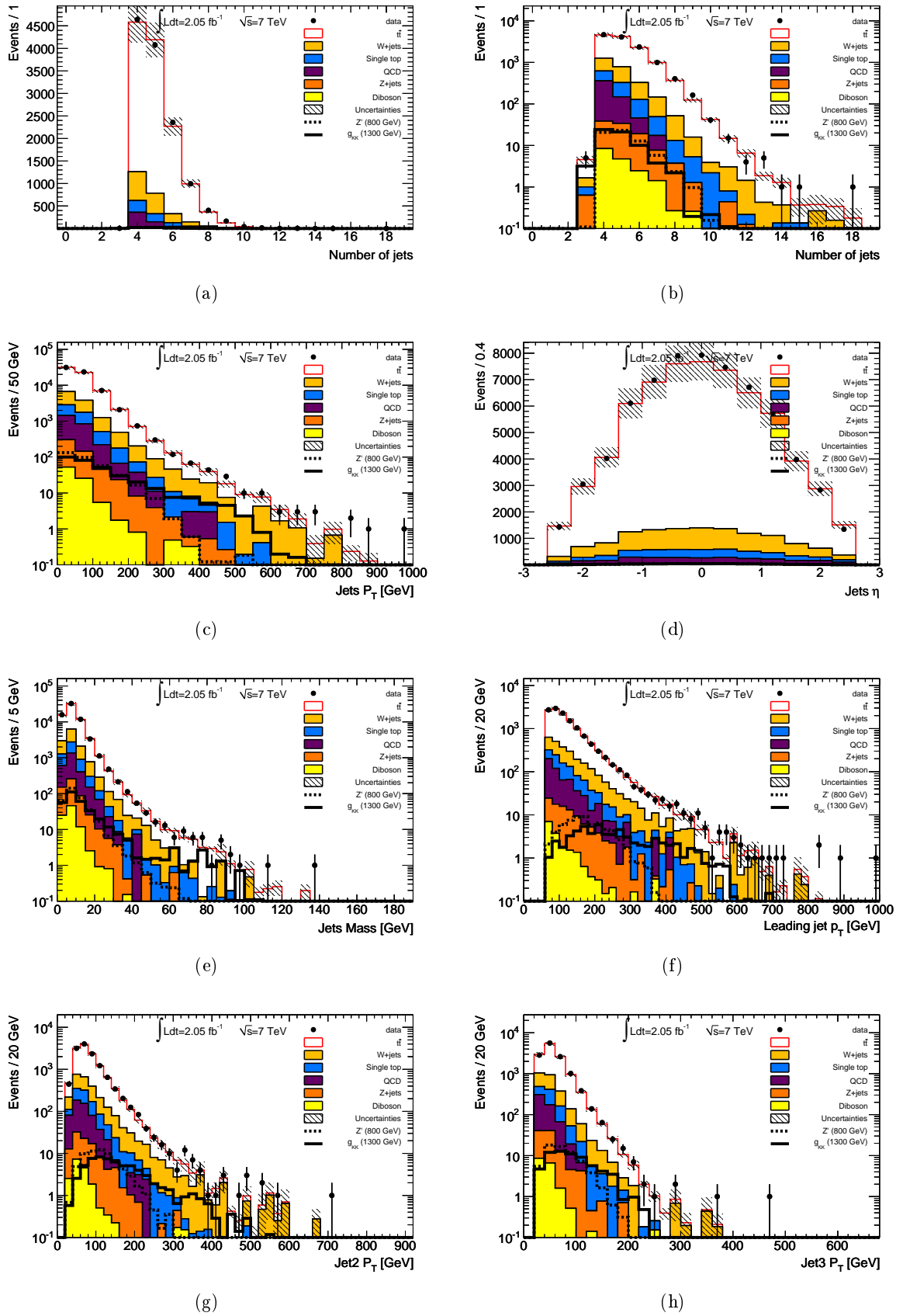
Figure E.2: Number of jets with p_T > 20 GeV in (a) linear and (b) logarithmic scales, jets (c) p_T , (d) \eta and (e) mass distributions, (f) leading jet p_T , (g) second jet p_T and (h) third jet p_T after all selection criteria were applied. The grey hashed area shows the total background normalization uncertainty.
