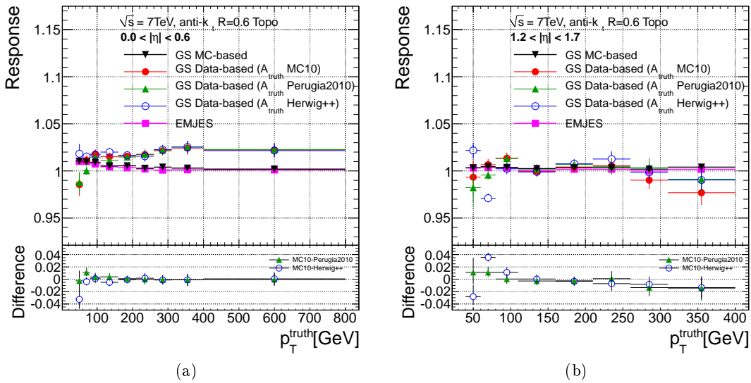
Figure 5.17: Average jet response calculated using the truth jet as a function of p_T^{\text{truth}} after applying GS corrections derived from the nominal PYTHIA sample (black triangles) and data using the A_{\text{truth}} calculated using the nominal PYTHIA MC10 (red circles), the Perugia2010 tune (green triangles) and the HERWIG++ sample (blue circles) for jets with (a) |\eta| < 0.6 and (b) 1.2 < |\eta| < 1.7 .
