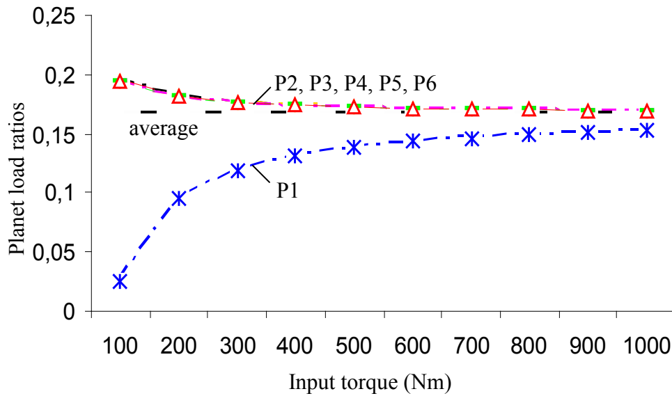
Figure 9 – 6-planet load ratios versus the input torque on the sun-gear
