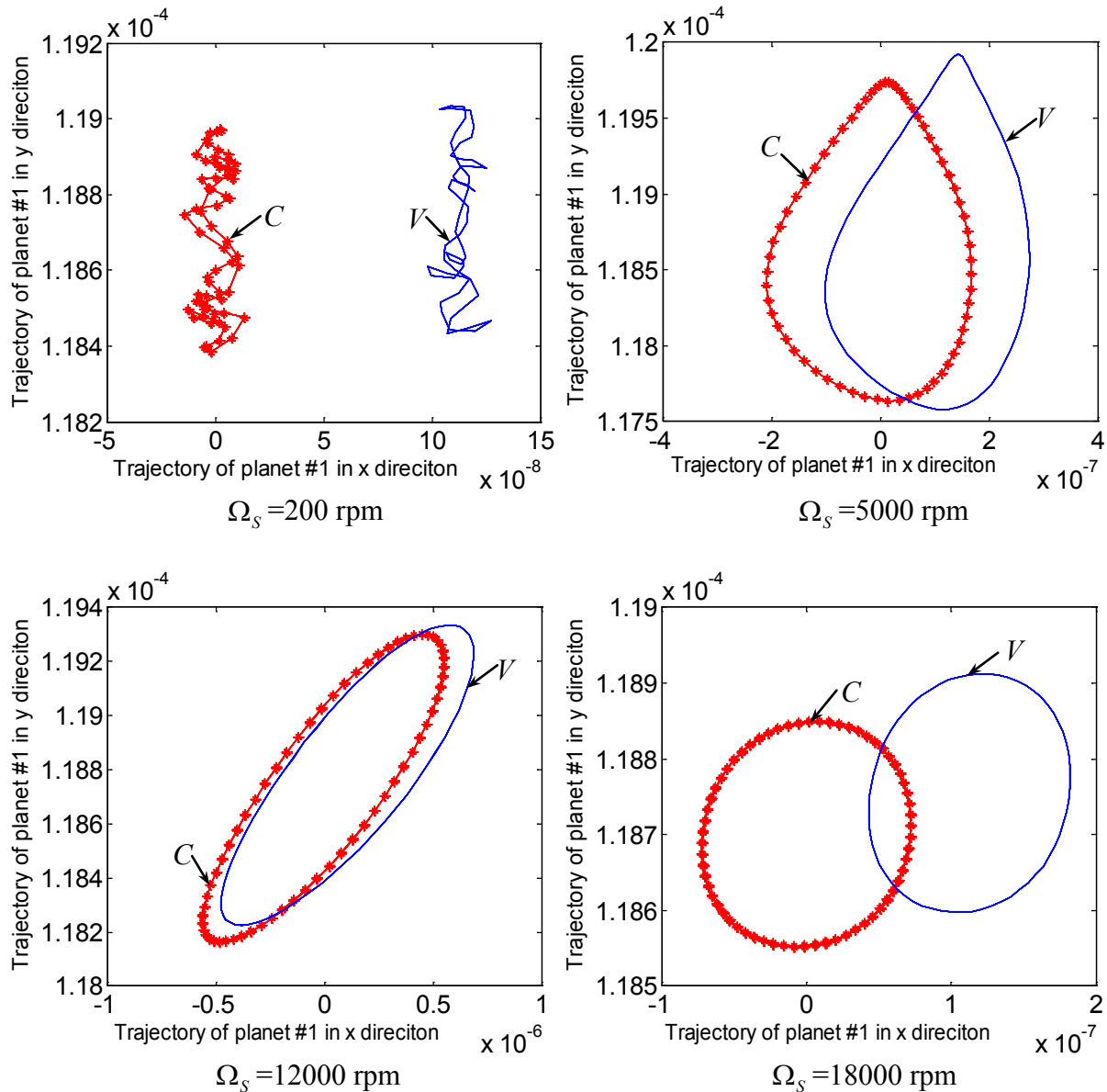
Figure 8-d – Trajectory of planet #1 at various speeds (fixed carrier, tangential position error ey_1 = -0.0002 m on planet #1)
