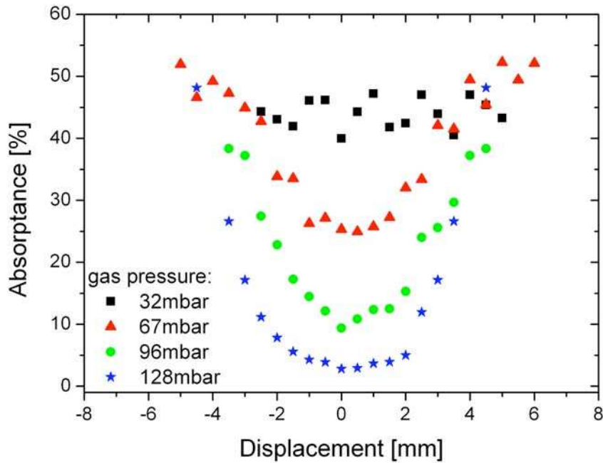
Fig. 3.5. Comparison between laser absorbance profiles collected for various ^3\text{He} gas pressures. The measurements were done at 2 T.
