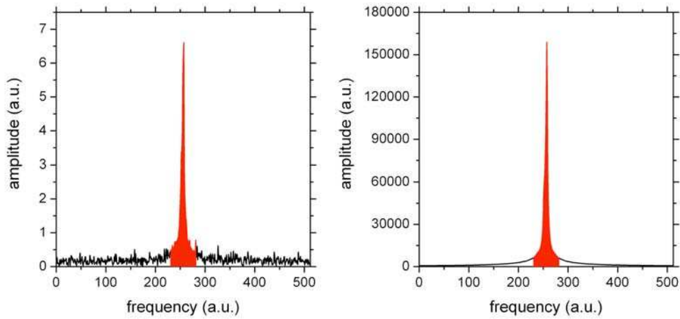
Fig. 4.14. FT of the absolute value of the FID signal (512 samples, 10 kHz bandwidth) obtained in the thermally polarized phantom (left, M = 3.892 \cdot 10^{-6} , P*V = 329.7 \pm 7 scc, flip angle: 61.6^\circ ) and the storage cell for the calibration experiment (right, P*V = 79,2 scc, flip angle: 61.6^\circ ). A comparison of the integrated signal under the peak (area in red under the curve) gave a polarization of 34.7 \pm 1.5\% .
