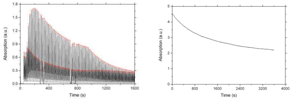
Fig. 4.6. Left: Absorption recorded during a multiscan acquisition of the probe doublet at 27 mbar. The pump laser was switched on at t = 86 s and switched off at t = 940 s. Although the ratios of the peaks induce a nice exponential build-up of the nuclear polarization, the total absorption decreases during the acquisition. Right: Absorption of a weak pump (channel CH0) tuned on f^{2m} transition. The decrease of absorption can not be explained by the OP process because of the small intensity used for this measurement.
