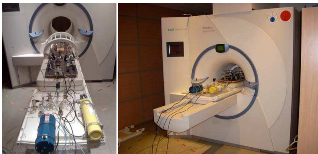
Fig. 4.13. Pictures of the high field polarizer outside (left) and inside the MRI scanner (right). The storage cell is in the center of the birdcage coil and the GHS is located at the bottom of the bed allowing access for a regulation of the flow during accumulation.
