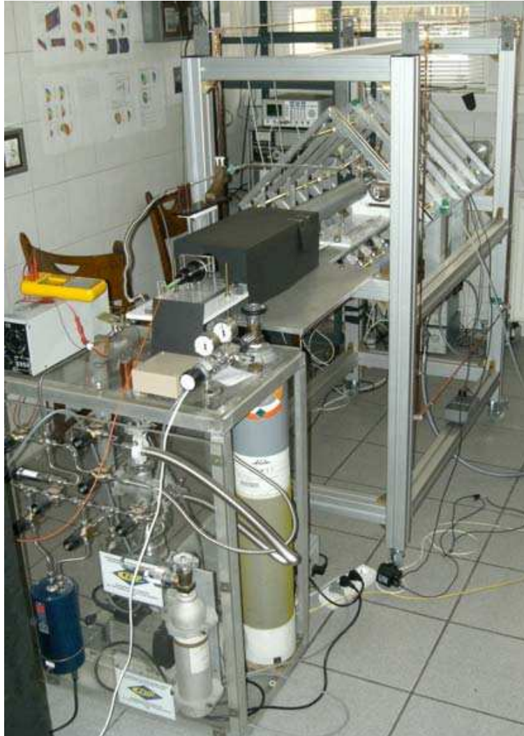
Fig. 2.2. Picture of the low field polarizer.
