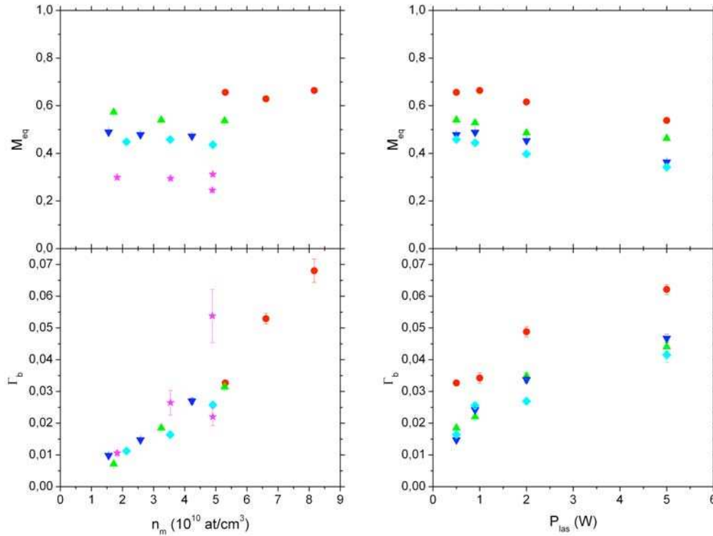
Fig. 3.23. Results obtained for 32 (circles), 67 (triangles), 96 (reversed triangles), 128 (diamonds) and 267 mbar (stars). Left: Steady-state polarization M_{\text{eq}} and build-up rate \Gamma_b as a function of n_m ( P_{\text{las}} = 0.5 W). Right: M_{\text{eq}} and \Gamma_b as a function of P_{\text{las}} . The influence of laser power was not performed at 267 mbar due to the difficulty to obtain stable discharges at this pressure.
