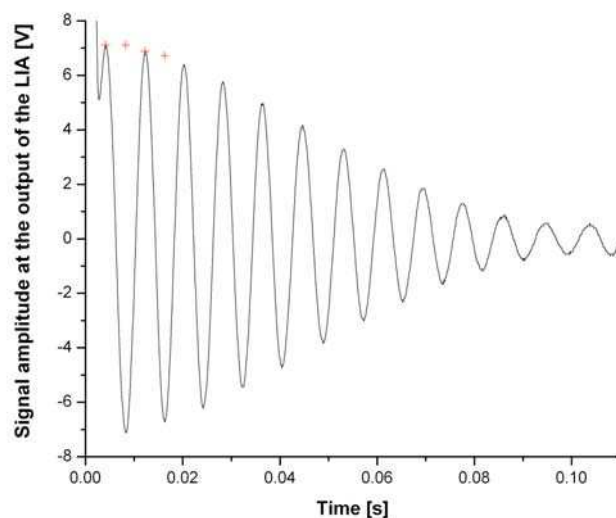
Fig. 2.11. FID signal recorded by the lock-in amplifier during a flip angle calibration and after a compression of polarized ^3\text{He} inside the small storage cell. The experiment lasted 6 min to reach a pressure of 57.8 mbar. At this pressure, the decay is not exponential and lasts around 100 ms. The starting amplitude was found with a linear fit of the peak to peak analysis of the 2 first oscillations. The flip angle was 45.9 \pm 0.5^\circ and the polarization 38.7 \pm 2\% .
