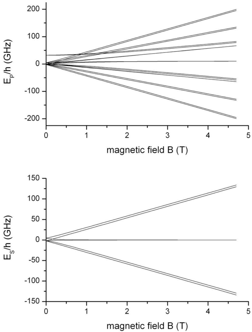
Fig. 1.6. Energy splits between sublevels in the metastable state 2^3S_1 (bottom) and first excited state 2^3P (top) as a function of the magnetic field B . The sublevels A_1 to A_6 and B_1 to B_{18} are labeled by their increasing order of energy and their energetic positions are defined so that their sum equals 0.
