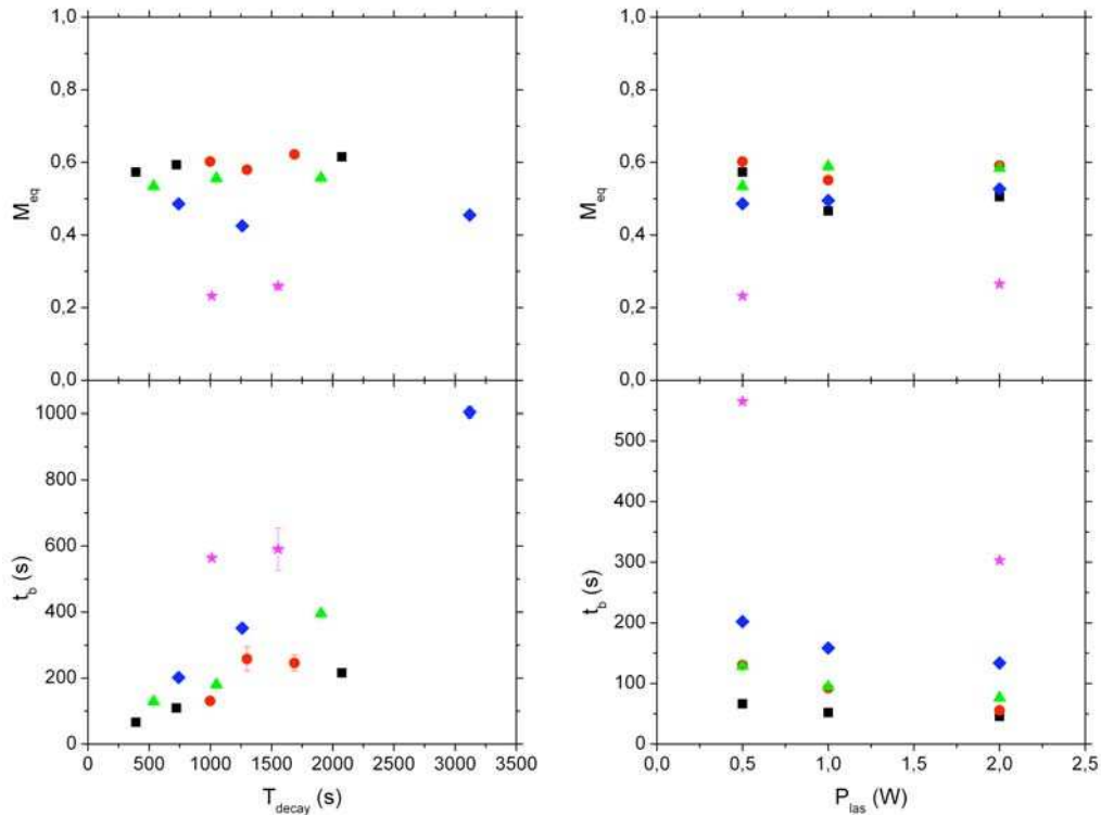
Fig. 3.17. Results obtained for 32 (squares), 67 (circles), 96 (triangles), 128 (diamonds) and 267 mbar (stars). Left: Steady-state polarization M_{\text{eq}} and build-up time t_b as a function of T_{\text{decay}} ( P_{\text{las}} = 0.5 W). Right: M_{\text{eq}} and t_b as a function of P_{\text{las}} . Only three acquisitions were done at 267 mbar due to the difficulty to obtain stable discharges at this pressure.
