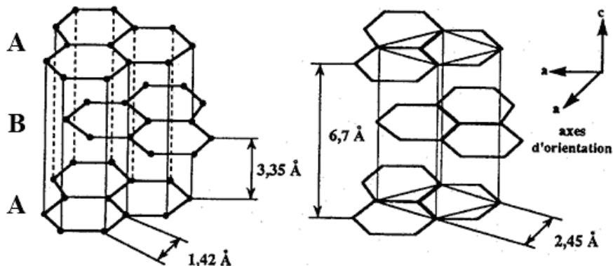
Figure 4-3: Structure cristallographique du graphite [22].
