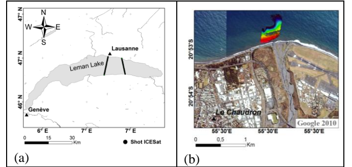
Fig. 2. (a) GLAS transects over Lemnan Lake, (b) HawkEye points across a coastal area in the northern part of Reunion Island.
