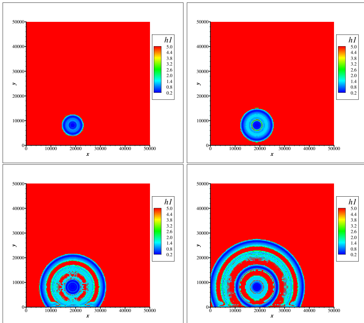
Fig. 9.19: 2D stroke model. Local reaction time steps h1 at 500 s (top left), 1000 s (top right), 2400 s (bottom left), and 3600 s (bottom right) within a half-splitting time step \Delta t/2 = 5 , represented on a dynamic adapted grid corresponding to 1024^2 points at the finest level J = 10 .
