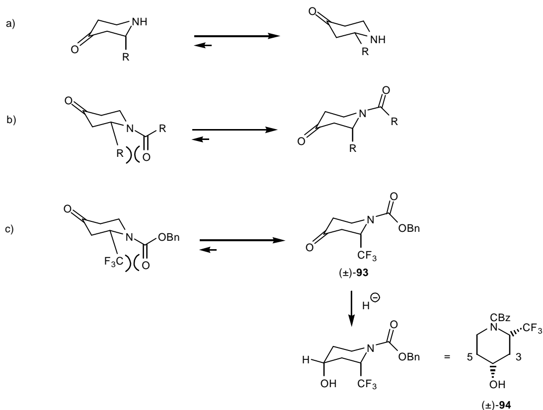
Scheme 26. Expected conformational equilibrium for: a) 2-substituted-4-piperidone free amines ; b) N -protected 2-substituted-4-piperidones ; c) carbamate ( \pm )- 93 .
