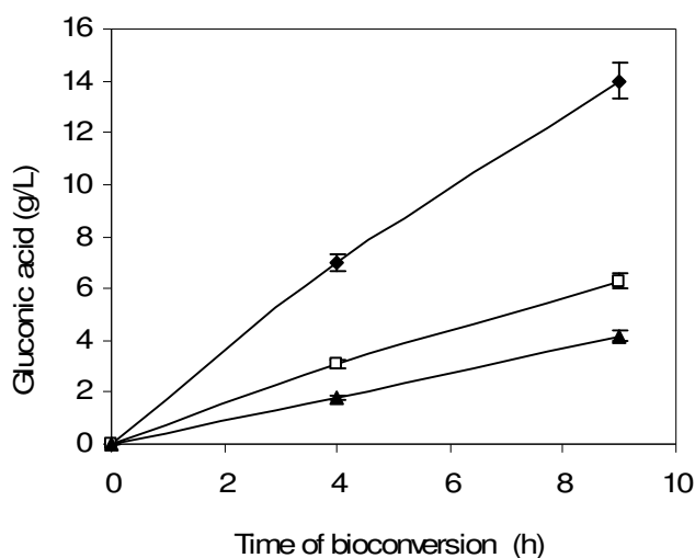
Fig 4.22. Effect of different temperatures ( \blacklozenge 60°C, \square 50°C, \blacktriangle 30°C) on biocatalytic activity of commercial glucose oxidase.
