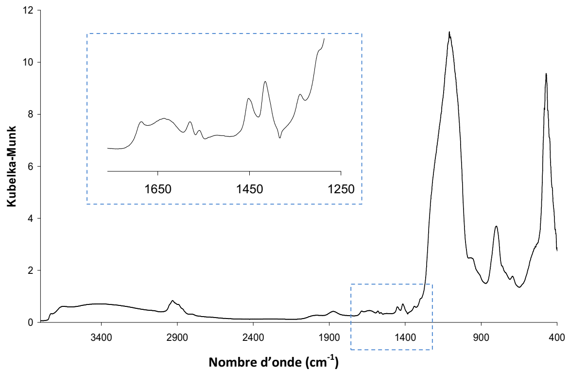
Figure 12 – Spectre DRIFT de la charge DSs
