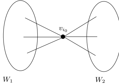
Figure 2.4: A 1-node-connected graph
