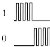
Figure II.49 – Codage Manchester
