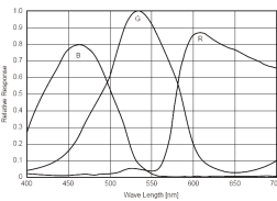
Sensor specifications b/w; color (extracted from the data sheet of the sensor - excluding lens and filter)
