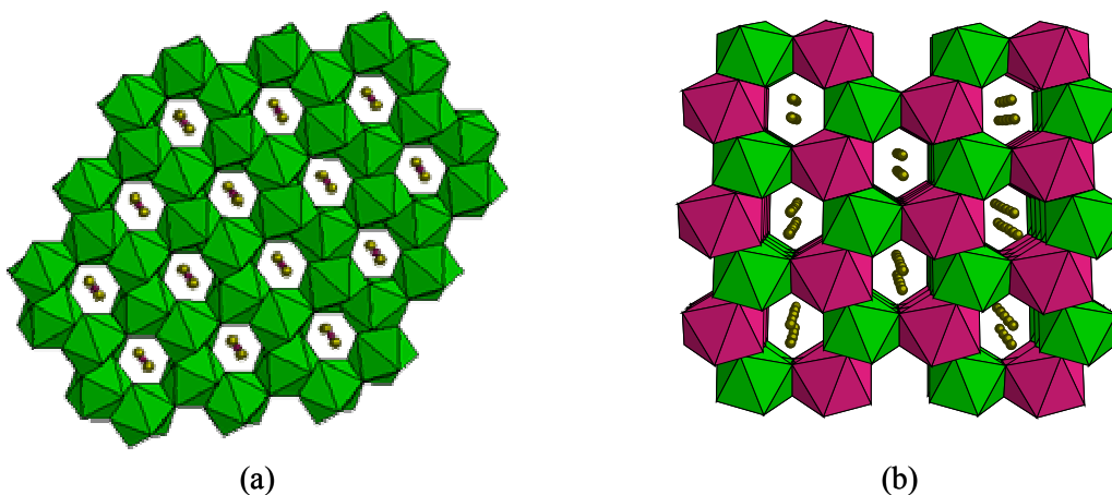
Figure III.9 : Structures de LiNaY_2F_8 (a) et LiYZrF_8 (b), isotypes de LiYTbF_8 .
