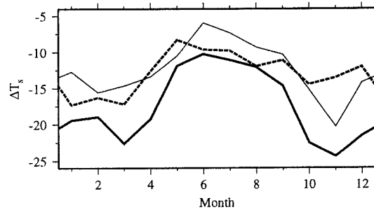
Figure 6.20: Monthly mean LGM-PD surface temperature difference (in °C). Thick line: GL21PC-GL0; thin line: GL21RC-GL0; dashed line: GL21PW-GL0.
